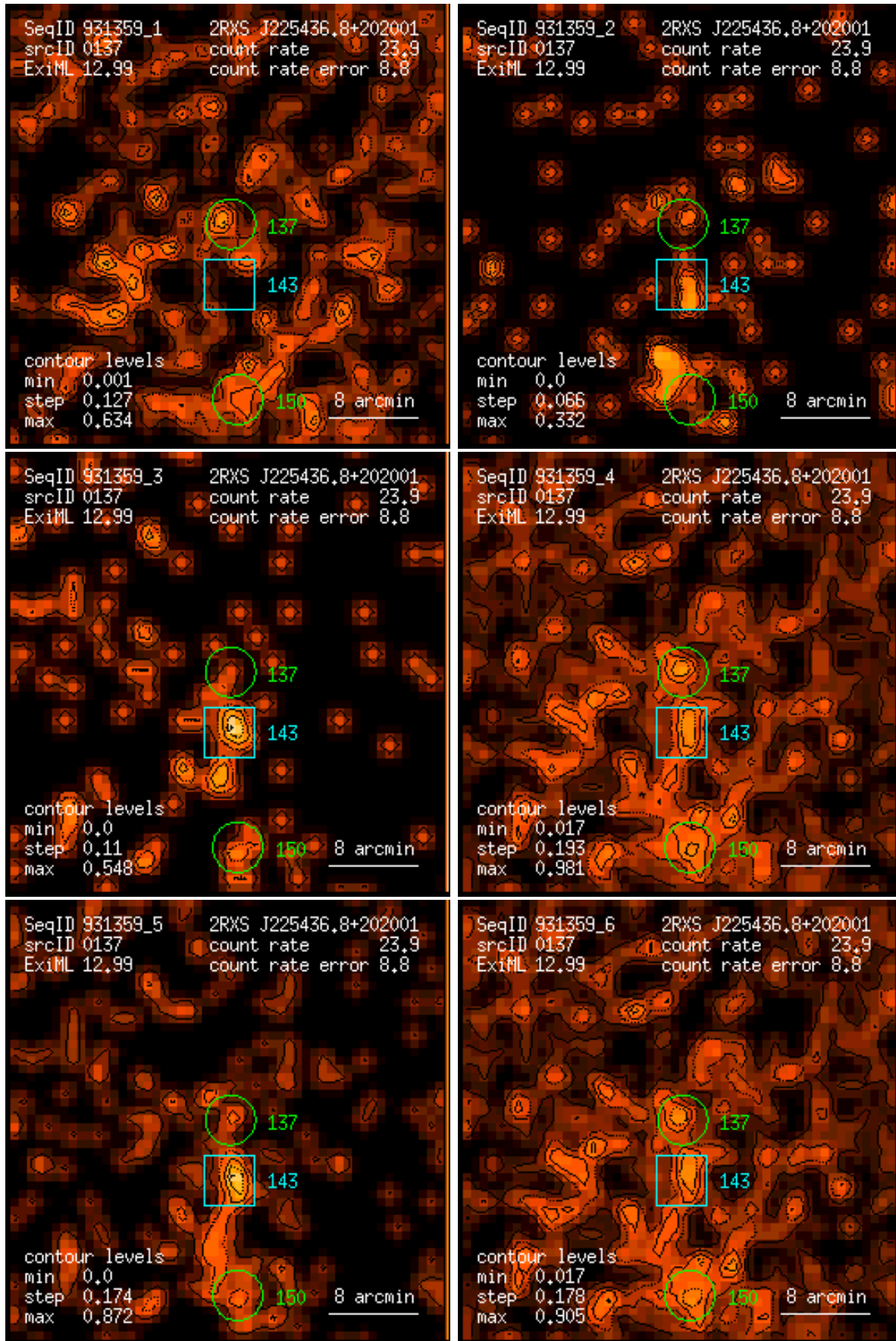
Figure 137: RASS 931359: detection 0137: band rate images, Gaussian filter: (1) PSPC channels 11 – 41, (2) 52 – 90, (3) 91 – 201, (4) 11 – 235, (5) 52 – 201, (6) 11 – 201. Broad band rates in counts/ks. Band rate contour levels in counts/ks/arcmin 2 .
