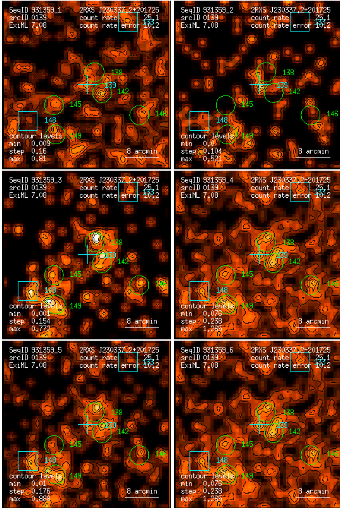
Figure 139: RASS 931359: detection 0139: band rate images, Gaussian filter: (1) PSPC channels 11 – 41, (2) 52 – 90, (3) 91 – 201, (4) 11 – 235, (5) 52 – 201, (6) 11 – 201. Broad band rates in counts/ks. Band rate contour levels in counts/ks/arcmin 2 .
