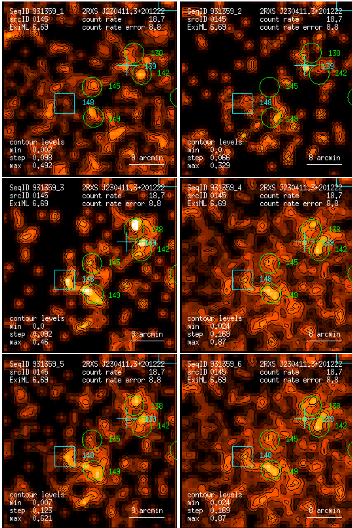
Figure 145: RASS 931359: detection 0145: band rate images, Gaussian filter: (1) PSPC channels 11 – 41, (2) 52 – 90, (3) 91 – 201, (4) 11 – 235, (5) 52 – 201, (6) 11 – 201. Broad band rates in counts/ks. Band rate contour levels in counts/ks/arcmin 2 .
