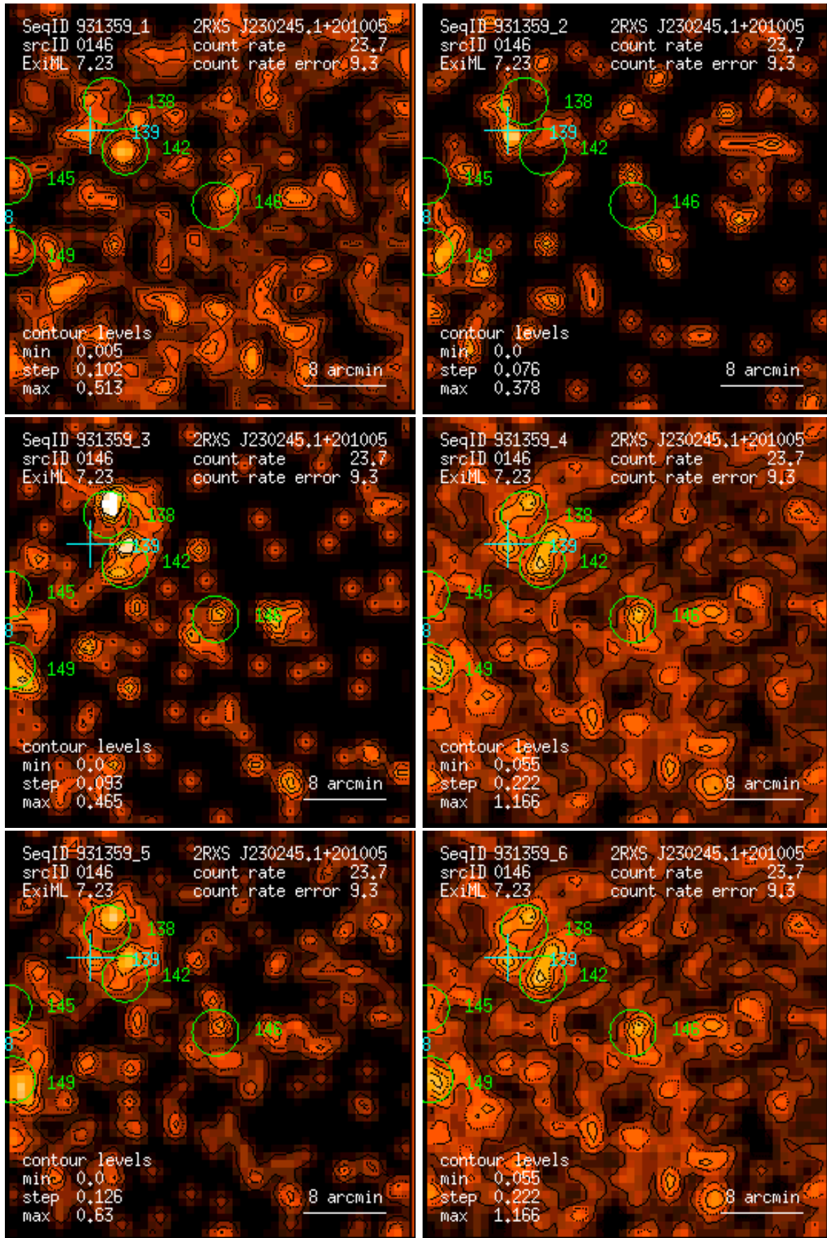
Figure 146: RASS 931359: detection 0146: band rate images, Gaussian filter: (1) PSPC channels 11 – 41, (2) 52 – 90, (3) 91 – 201, (4) 11 – 235, (5) 52 – 201, (6) 11 – 201. Broad band rates in counts/ks. Band rate contour levels in counts/ks/arcmin 2 .
