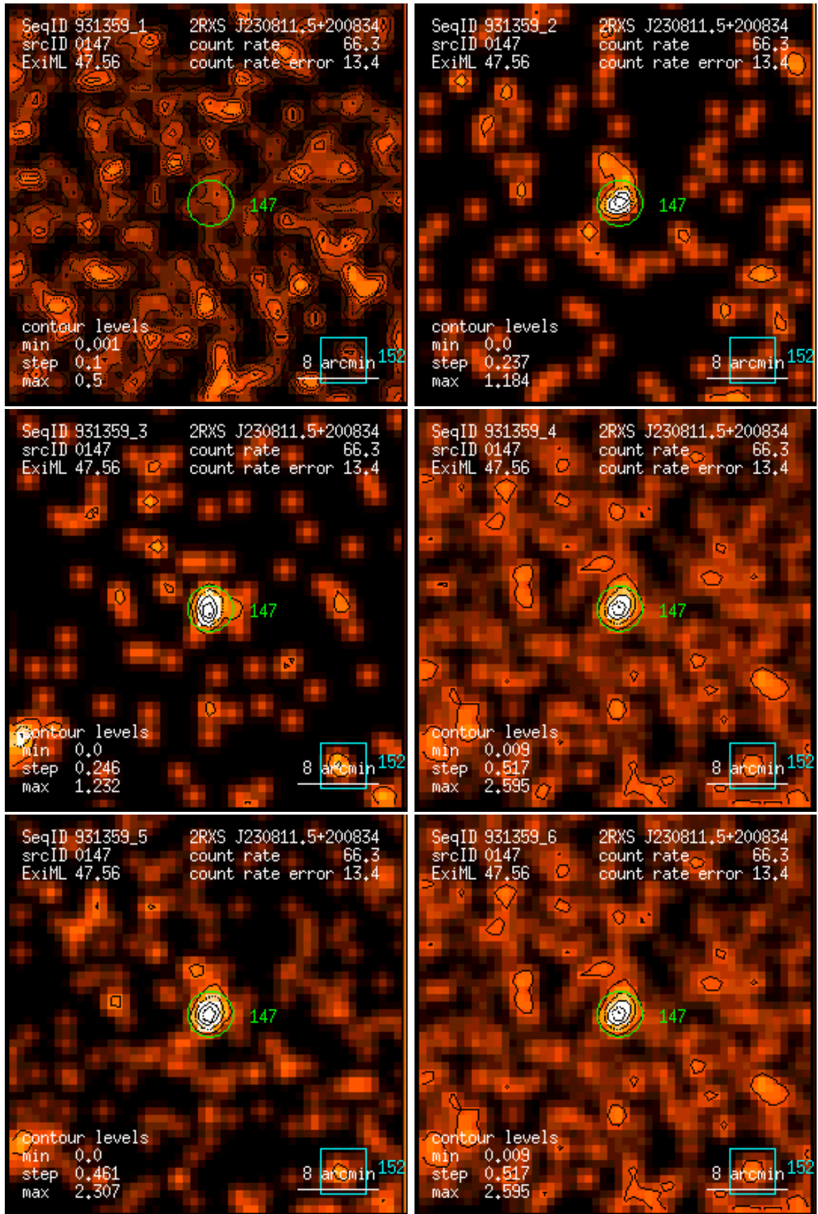
Figure 147: RASS 931359: detection 0147: band rate images, Gaussian filter: (1) PSPC channels 11 – 41, (2) 52 – 90, (3) 91 – 201, (4) 11 – 235, (5) 52 – 201, (6) 11 – 201. Broad band rates in counts/ks. Band rate contour levels in counts/ks/arcmin 2 .
