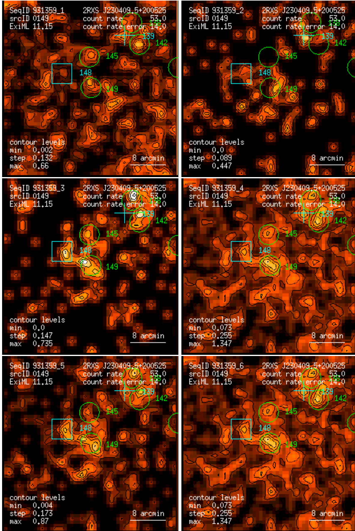
Figure 149: RASS 931359: detection 0149: band rate images, Gaussian filter: (1) PSPC channels 11 – 41, (2) 52 – 90, (3) 91 – 201, (4) 11 – 235, (5) 52 – 201, (6) 11 – 201. Broad band rates in counts/ks. Band rate contour levels in counts/ks/arcmin 2 .
