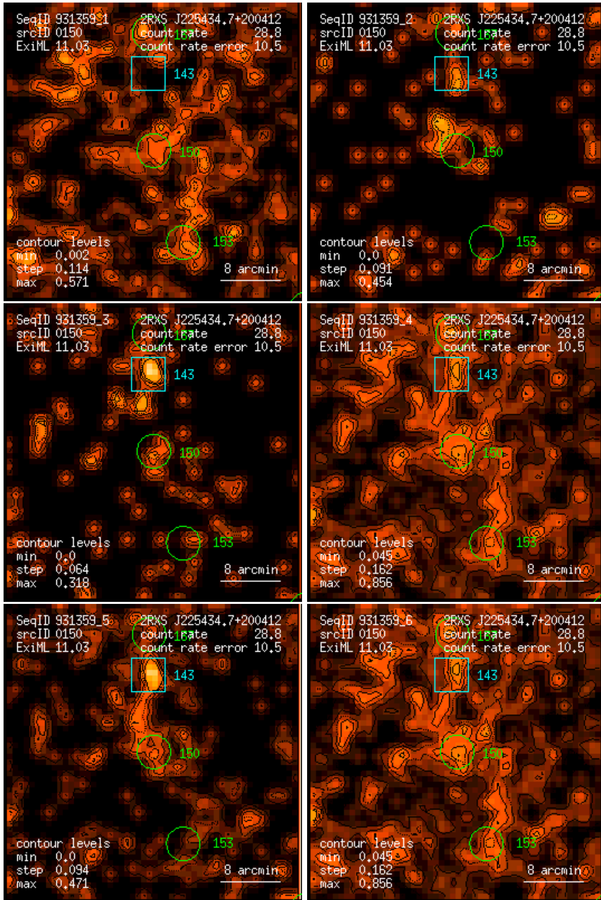
Figure 150: RASS 931359: detection 0150: band rate images, Gaussian filter: (1) PSPC channels 11 – 41, (2) 52 – 90, (3) 91 – 201, (4) 11 – 235, (5) 52 – 201, (6) 11 – 201. Broad band rates in counts/ks. Band rate contour levels in counts/ks/arcmin 2 .
