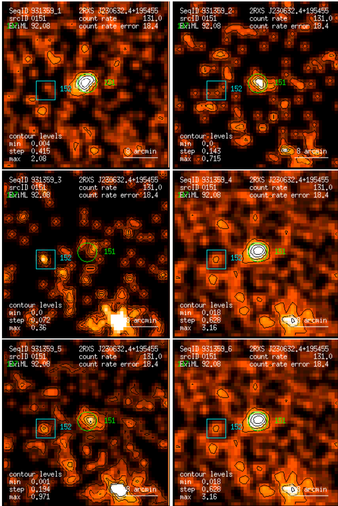
Figure 151: RASS 931359: detection 0151: band rate images, Gaussian filter: (1) PSPC channels 11 – 41, (2) 52 – 90, (3) 91 – 201, (4) 11 – 235, (5) 52 – 201, (6) 11 – 201. Broad band rates in counts/ks. Band rate contour levels in counts/ks/arcmin 2 .
