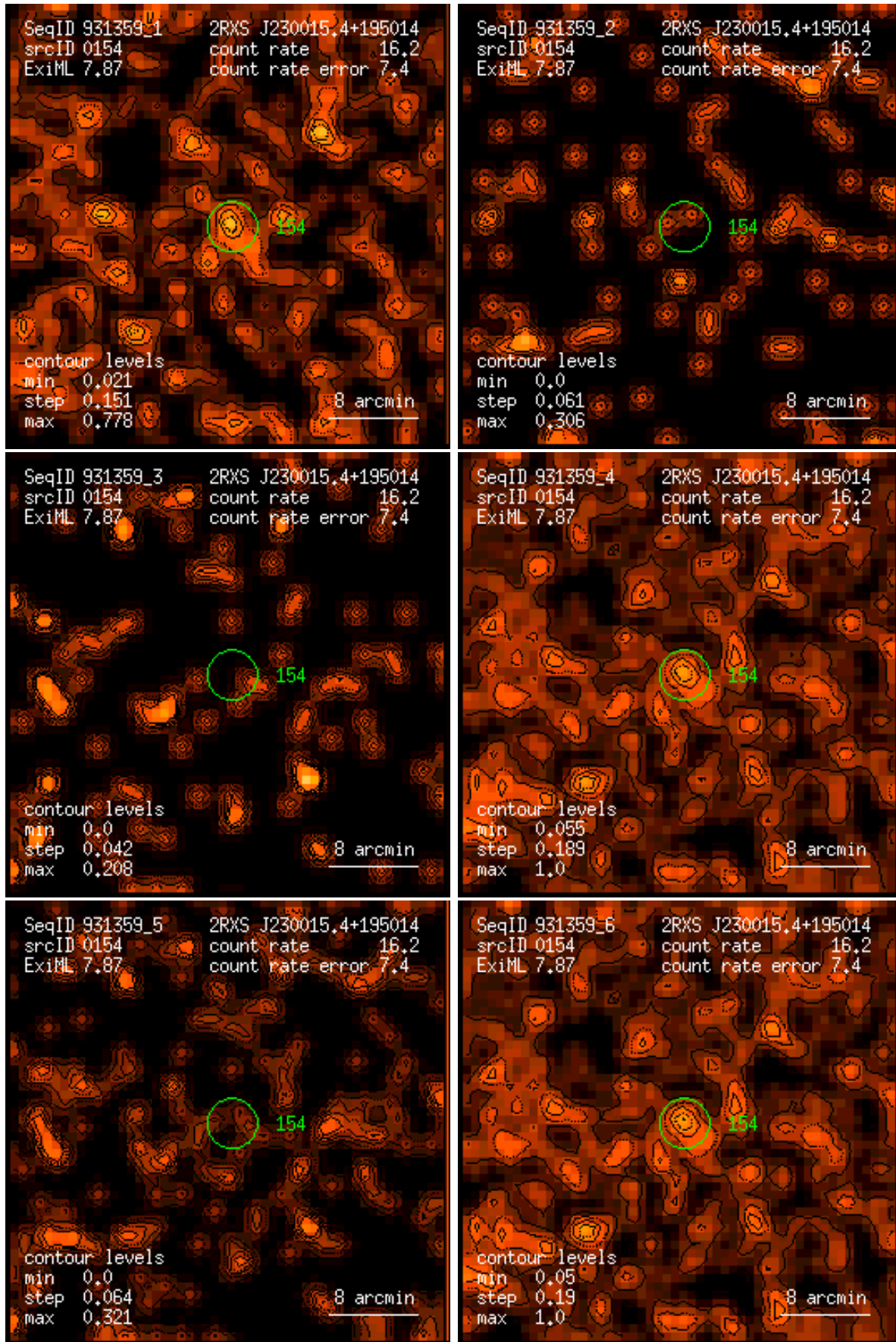
Figure 154: RASS 931359: detection 0154: band rate images, Gaussian filter: (1) PSPC channels 11 – 41, (2) 52 – 90, (3) 91 – 201, (4) 11 – 235, (5) 52 – 201, (6) 11 – 201. Broad band rates in counts/ks. Band rate contour levels in counts/ks/arcmin 2 .
