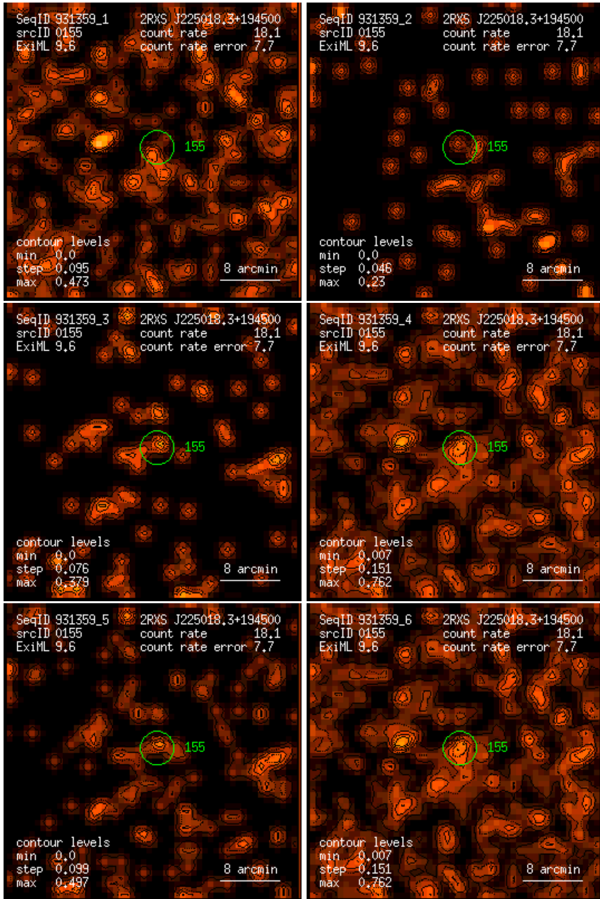
Figure 155: RASS 931359: detection 0155: band rate images, Gaussian filter: (1) PSPC channels 11 – 41, (2) 52 – 90, (3) 91 – 201, (4) 11 – 235, (5) 52 – 201, (6) 11 – 201. Broad band rates in counts/ks. Band rate contour levels in counts/ks/arcmin 2 .
