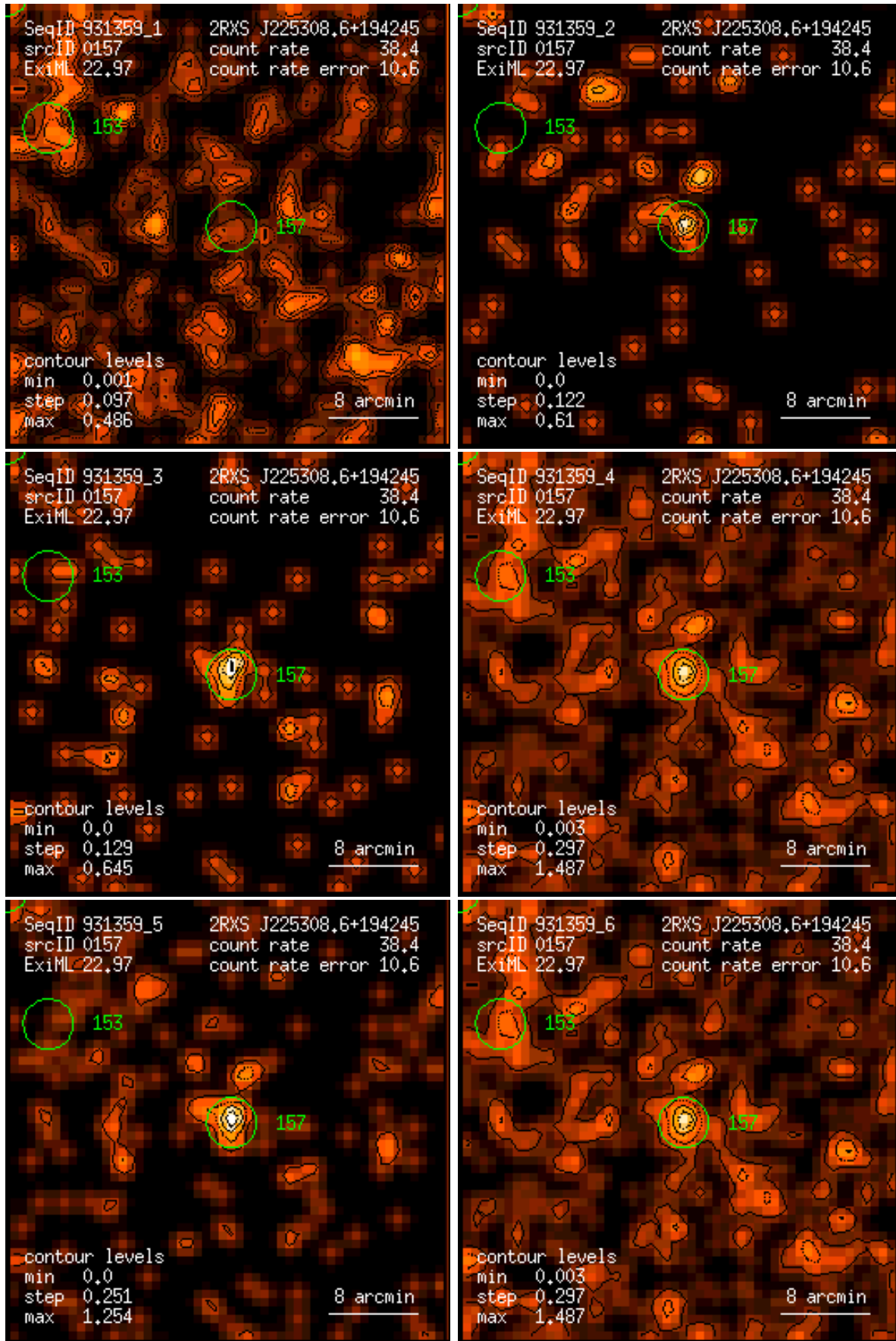
Figure 157: RASS 931359: detection 0157: band rate images, Gaussian filter: (1) PSPC channels 11 – 41, (2) 52 – 90, (3) 91 – 201, (4) 11 – 235, (5) 52 – 201, (6) 11 – 201. Broad band rates in counts/ks. Band rate contour levels in counts/ks/arcmin 2 .
