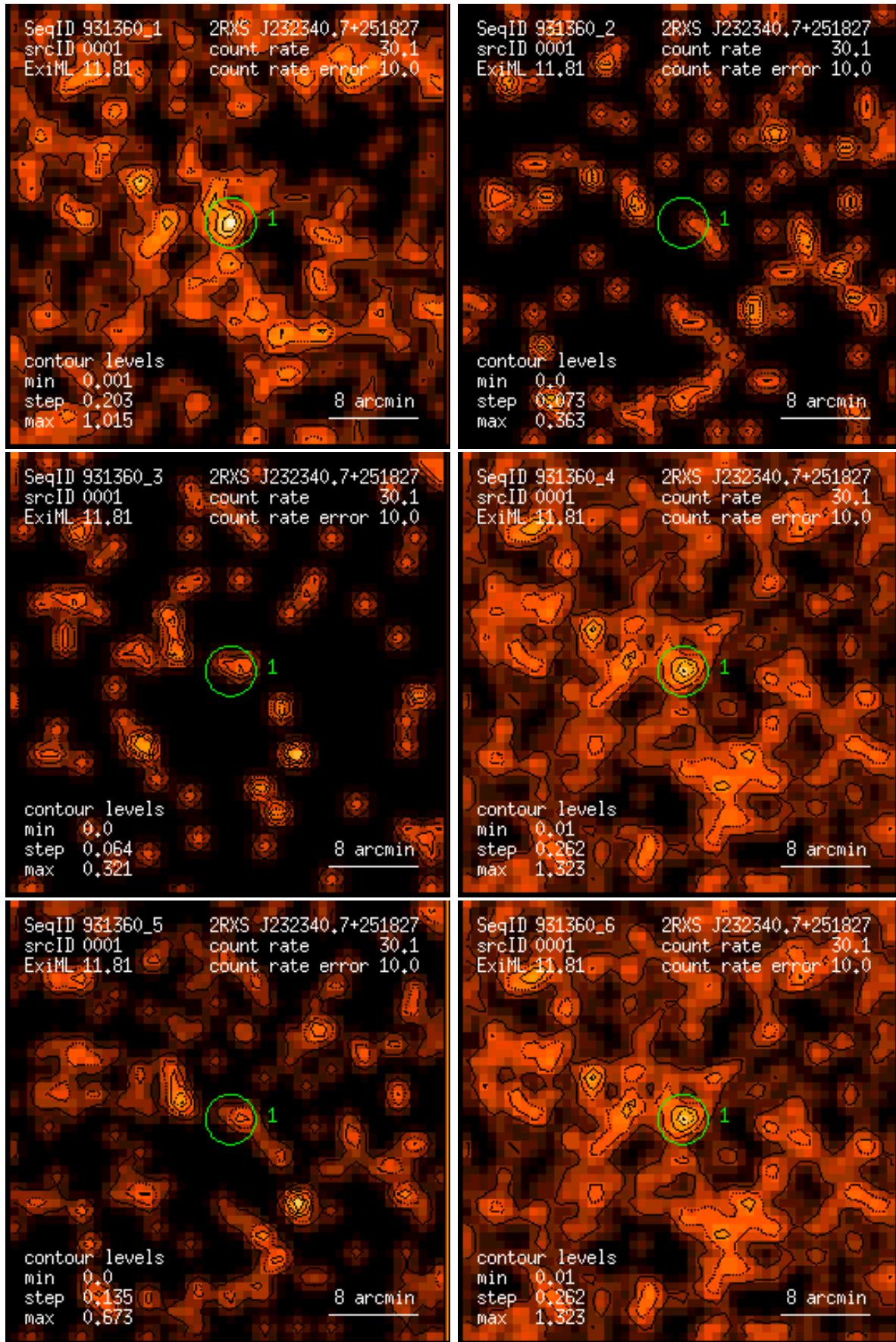
Figure 1: RASS 931360: detection 0001: band rate images, Gaussian filter: (1) PSPC channels 11 – 41, (2) 52 – 90, (3) 91 – 201, (4) 11 – 235, (5) 52 – 201, (6) 11 – 201. Broad band rates in counts/ks. Band rate contour levels in counts/ks/arcmin 2 .
