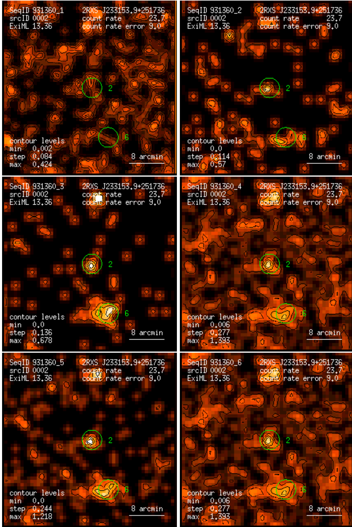
Figure 2: RASS 931360: detection 0002: band rate images, Gaussian filter: (1) PSPC channels 11 – 41, (2) 52 – 90, (3) 91 – 201, (4) 11 – 235, (5) 52 – 201, (6) 11 – 201. Broad band rates in counts/ks. Band rate contour levels in counts/ks/arcmin 2 .
