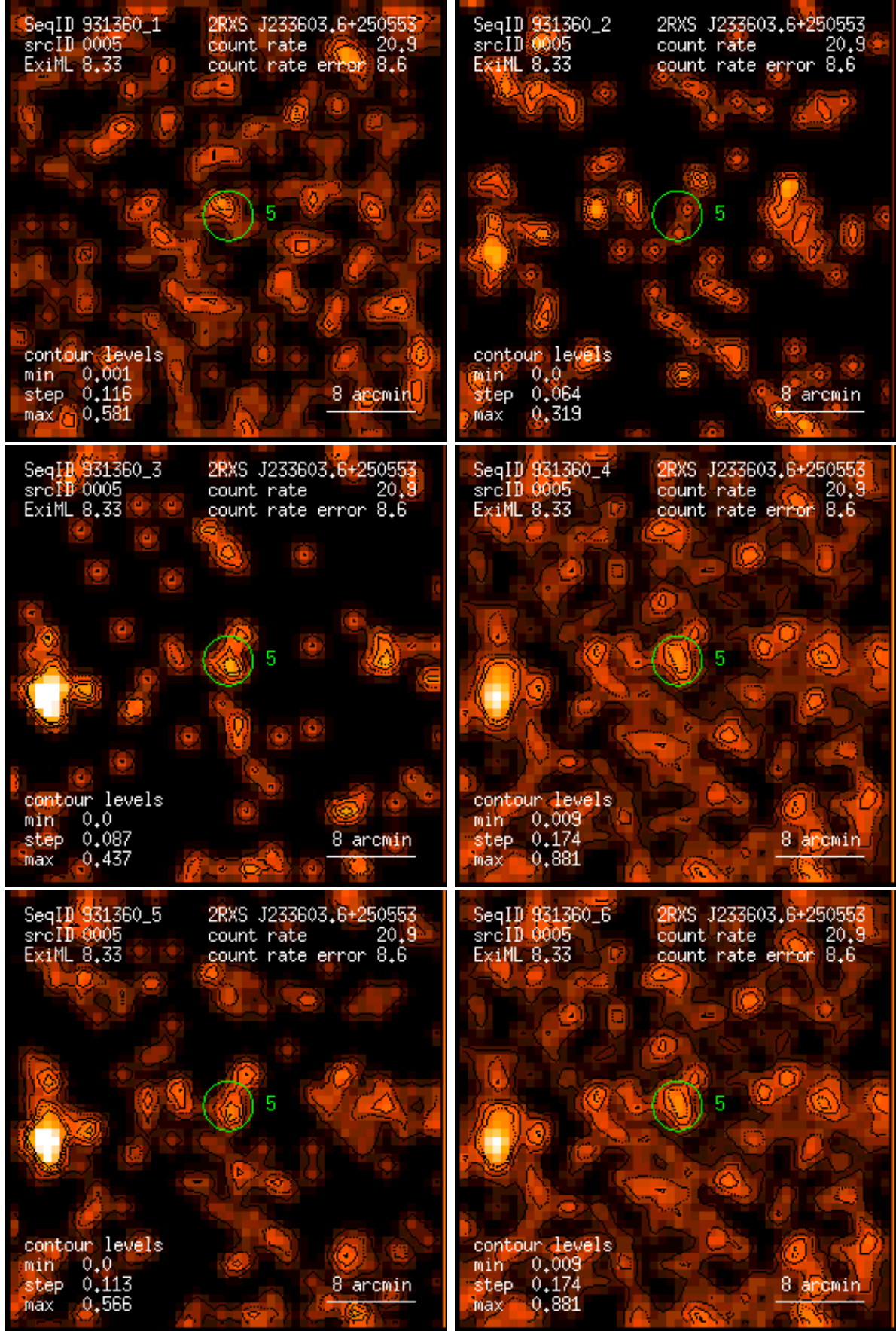
Figure 5: RASS 931360: detection 0005: band rate images, Gaussian filter: (1) PSPC channels 11 – 41, (2) 52 – 90, (3) 91 – 201, (4) 11 – 235, (5) 52 – 201, (6) 11 – 201. Broad band rates in counts/ks. Band rate contour levels in counts/ks/arcmin 2 .
