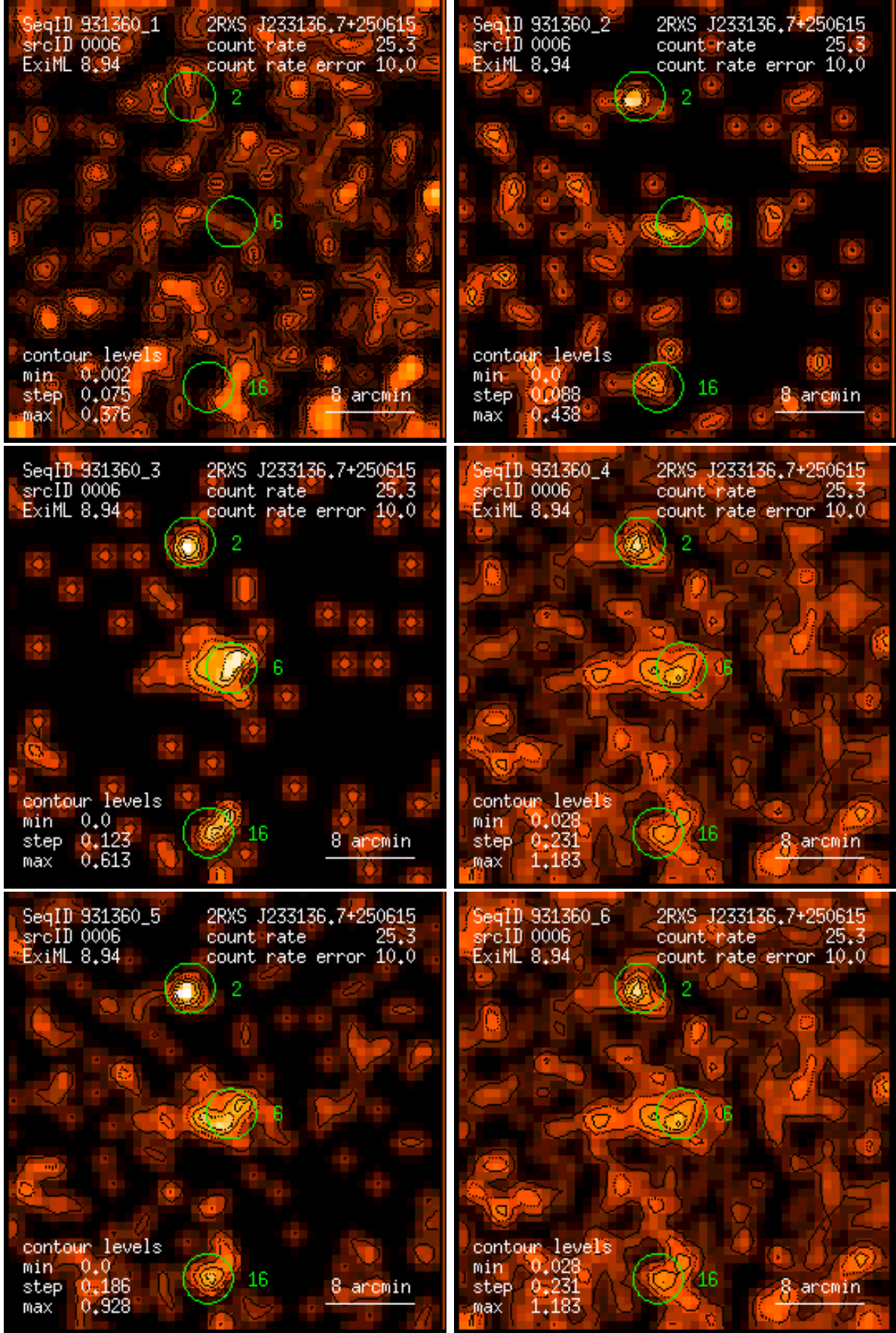
Figure 6: RASS 931360: detection 0006: band rate images, Gaussian filter: (1) PSPC channels 11 – 41, (2) 52 – 90, (3) 91 – 201, (4) 11 – 235, (5) 52 – 201, (6) 11 – 201. Broad band rates in counts/ks. Band rate contour levels in counts/ks/arcmin 2 .
