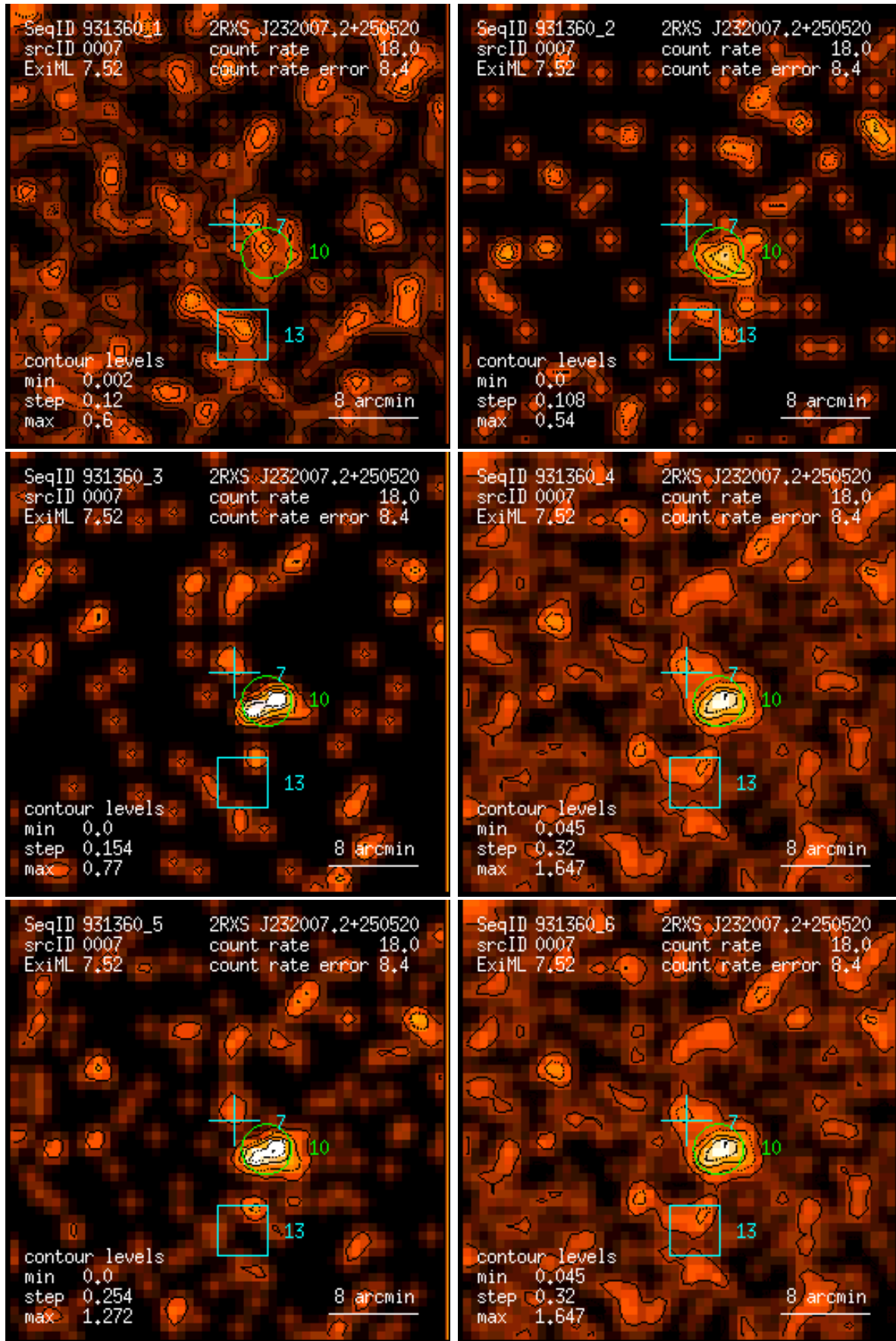
Figure 7: RASS 931360: detection 0007: band rate images, Gaussian filter: (1) PSPC channels 11 – 41, (2) 52 – 90, (3) 91 – 201, (4) 11 – 235, (5) 52 – 201, (6) 11 – 201. Broad band rates in counts/ks. Band rate contour levels in counts/ks/arcmin 2 .
