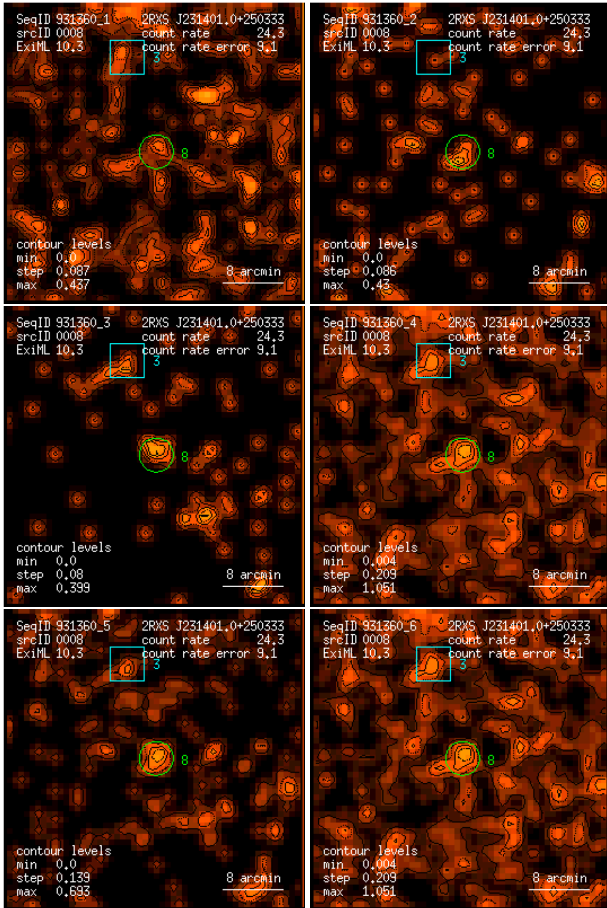
Figure 8: RASS 931360: detection 0008: band rate images, Gaussian filter: (1) PSPC channels 11 – 41, (2) 52 – 90, (3) 91 – 201, (4) 11 – 235, (5) 52 – 201, (6) 11 – 201. Broad band rates in counts/ks. Band rate contour levels in counts/ks/arcmin 2 .
