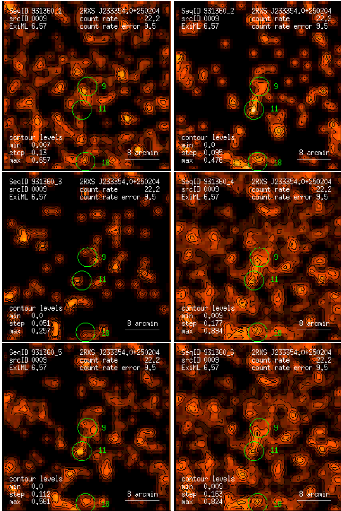
Figure 9: RASS 931360: detection 0009: band rate images, Gaussian filter: (1) PSPC channels 11 – 41, (2) 52 – 90, (3) 91 – 201, (4) 11 – 235, (5) 52 – 201, (6) 11 – 201. Broad band rates in counts/ks. Band rate contour levels in counts/ks/arcmin 2 .
