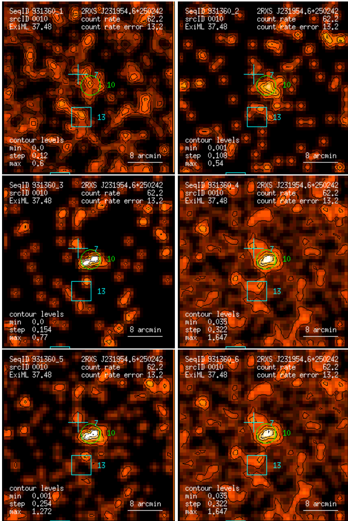
Figure 10: RASS 931360: detection 0010: band rate images, Gaussian filter: (1) PSPC channels 11 – 41, (2) 52 – 90, (3) 91 – 201, (4) 11 – 235, (5) 52 – 201, (6) 11 – 201. Broad band rates in counts/ks. Band rate contour levels in counts/ks/arcmin 2 .
