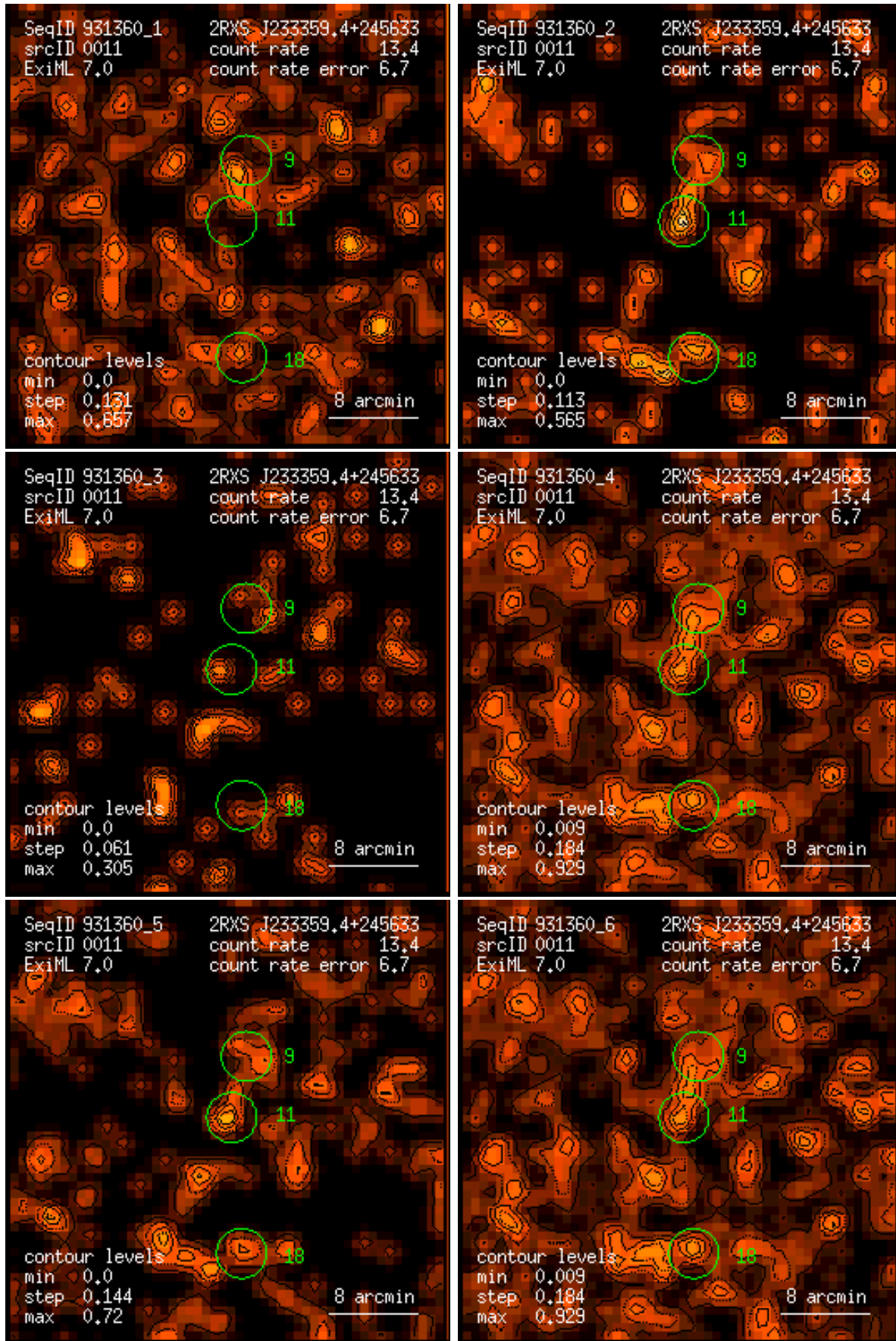
Figure 11: RASS 931360: detection 0011: band rate images, Gaussian filter: (1) PSPC channels 11 – 41, (2) 52 – 90, (3) 91 – 201, (4) 11 – 235, (5) 52 – 201, (6) 11 – 201. Broad band rates in counts/ks. Band rate contour levels in counts/ks/arcmin 2 .
