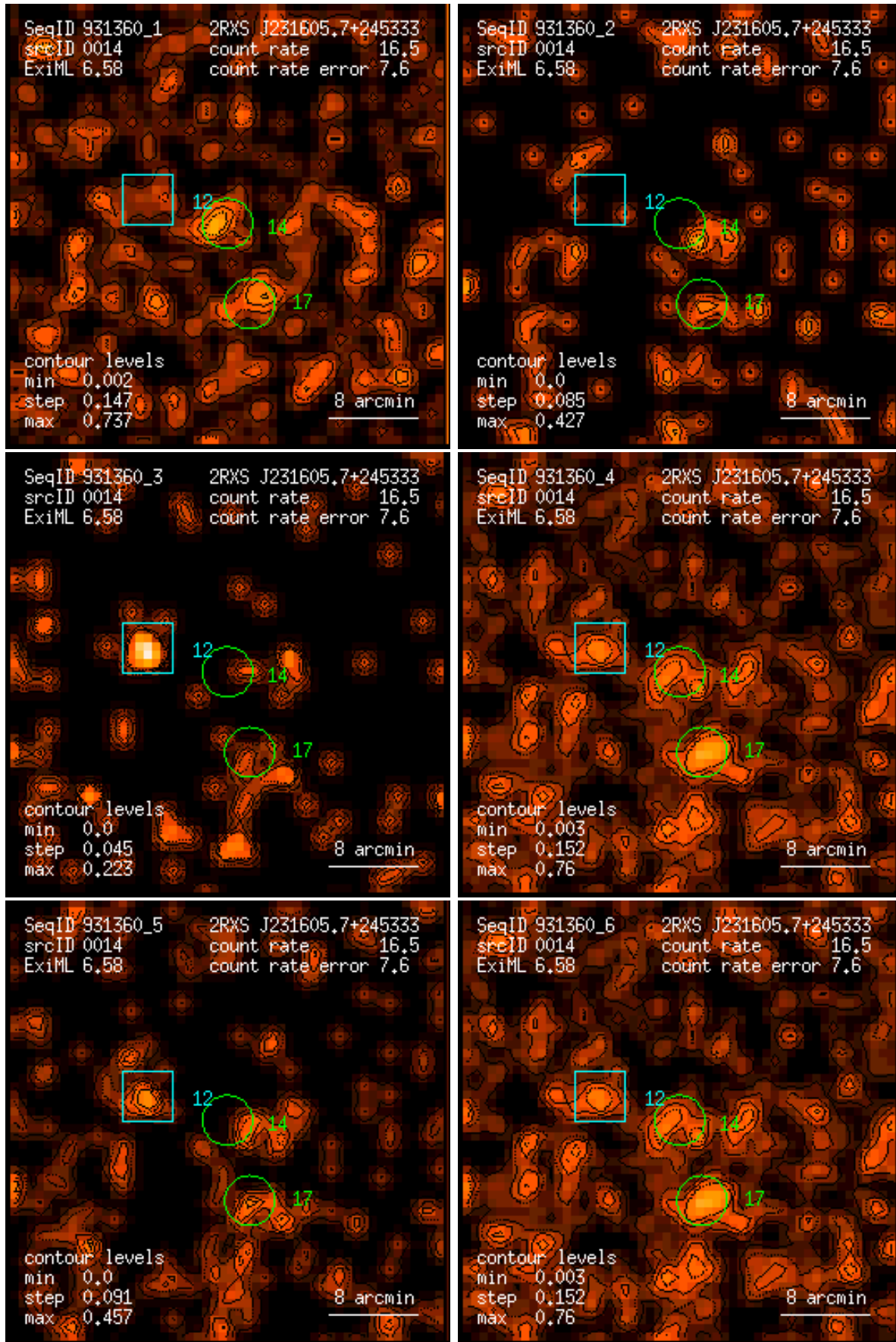
Figure 14: RASS 931360: detection 0014: band rate images, Gaussian filter: (1) PSPC channels 11 – 41, (2) 52 – 90, (3) 91 – 201, (4) 11 – 235, (5) 52 – 201, (6) 11 – 201. Broad band rates in counts/ks. Band rate contour levels in counts/ks/arcmin 2 .
