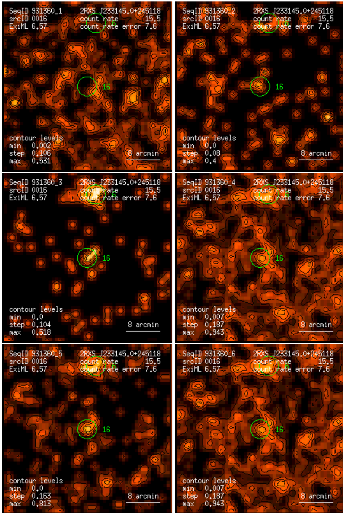
Figure 16: RASS 931360: detection 0016: band rate images, Gaussian filter: (1) PSPC channels 11 – 41, (2) 52 – 90, (3) 91 – 201, (4) 11 – 235, (5) 52 – 201, (6) 11 – 201. Broad band rates in counts/ks. Band rate contour levels in counts/ks/arcmin 2 .
