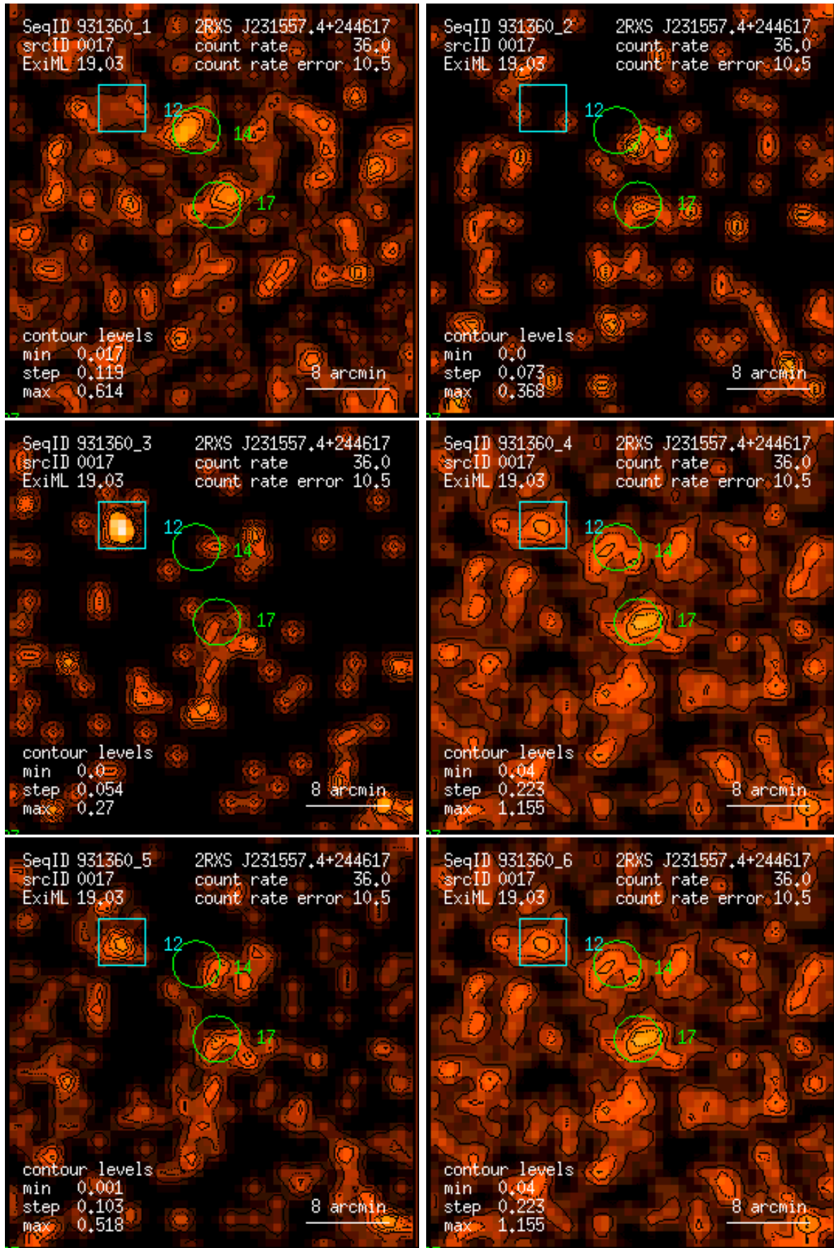
Figure 17: RASS 931360: detection 0017: band rate images, Gaussian filter: (1) PSPC channels 11 – 41, (2) 52 – 90, (3) 91 – 201, (4) 11 – 235, (5) 52 – 201, (6) 11 – 201. Broad band rates in counts/ks. Band rate contour levels in counts/ks/arcmin 2 .
