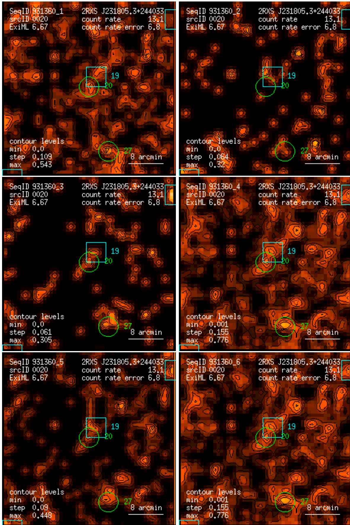
Figure 20: RASS 931360: detection 0020: band rate images, Gaussian filter: (1) PSPC channels 11 – 41, (2) 52 – 90, (3) 91 – 201, (4) 11 – 235, (5) 52 – 201, (6) 11 – 201. Broad band rates in counts/ks. Band rate contour levels in counts/ks/arcmin 2 .
