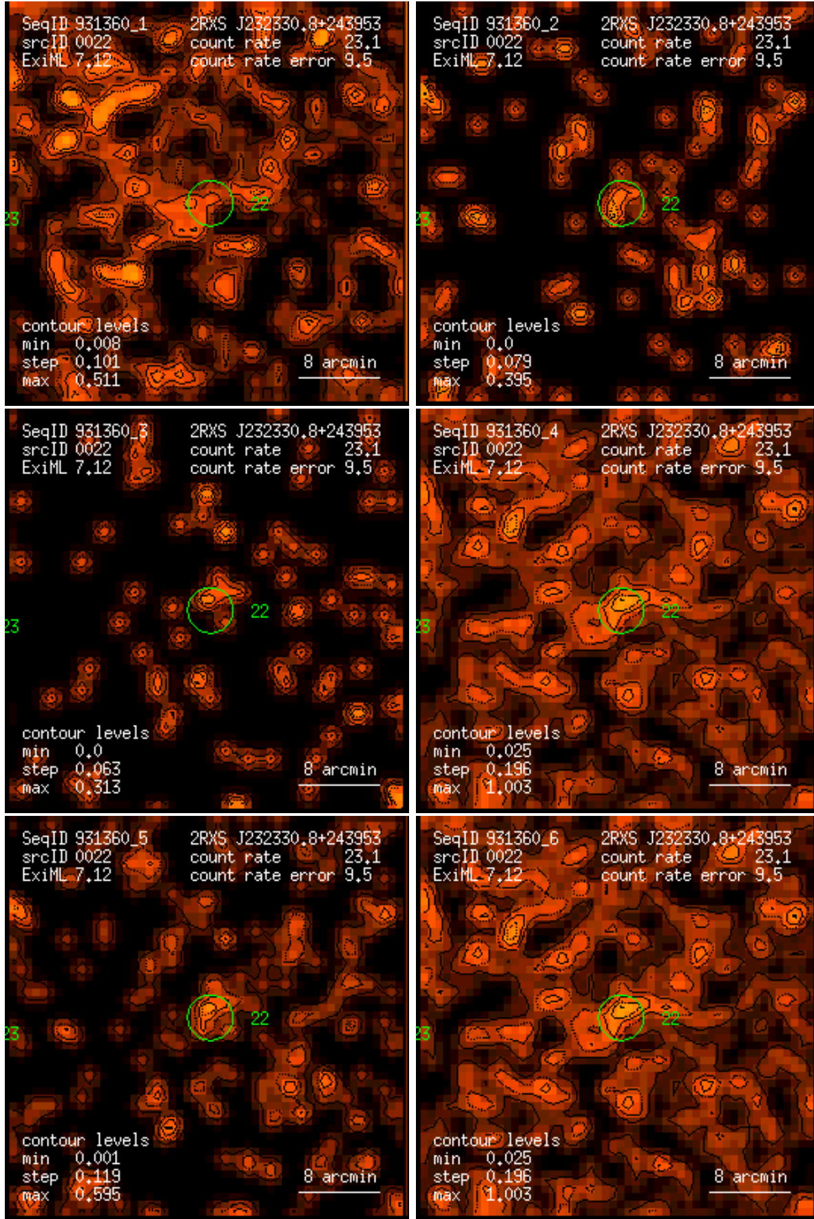
Figure 22: RASS 931360: detection 0022: band rate images, Gaussian filter: (1) PSPC channels 11 – 41, (2) 52 – 90, (3) 91 – 201, (4) 11 – 235, (5) 52 – 201, (6) 11 – 201. Broad band rates in counts/ks. Band rate contour levels in counts/ks/arcmin 2 .
