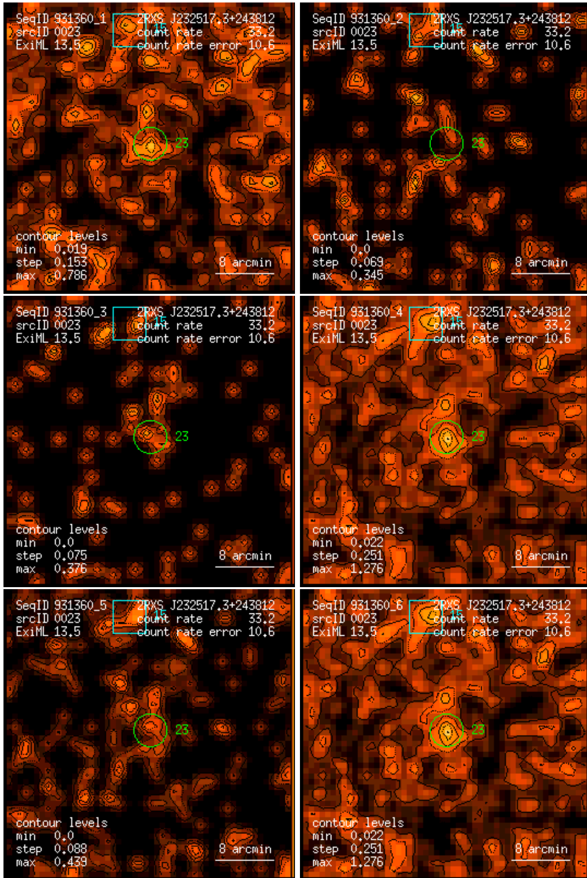
Figure 23: RASS 931360: detection 0023: band rate images, Gaussian filter: (1) PSPC channels 11 – 41, (2) 52 – 90, (3) 91 – 201, (4) 11 – 235, (5) 52 – 201, (6) 11 – 201. Broad band rates in counts/ks. Band rate contour levels in counts/ks/arcmin 2 .
