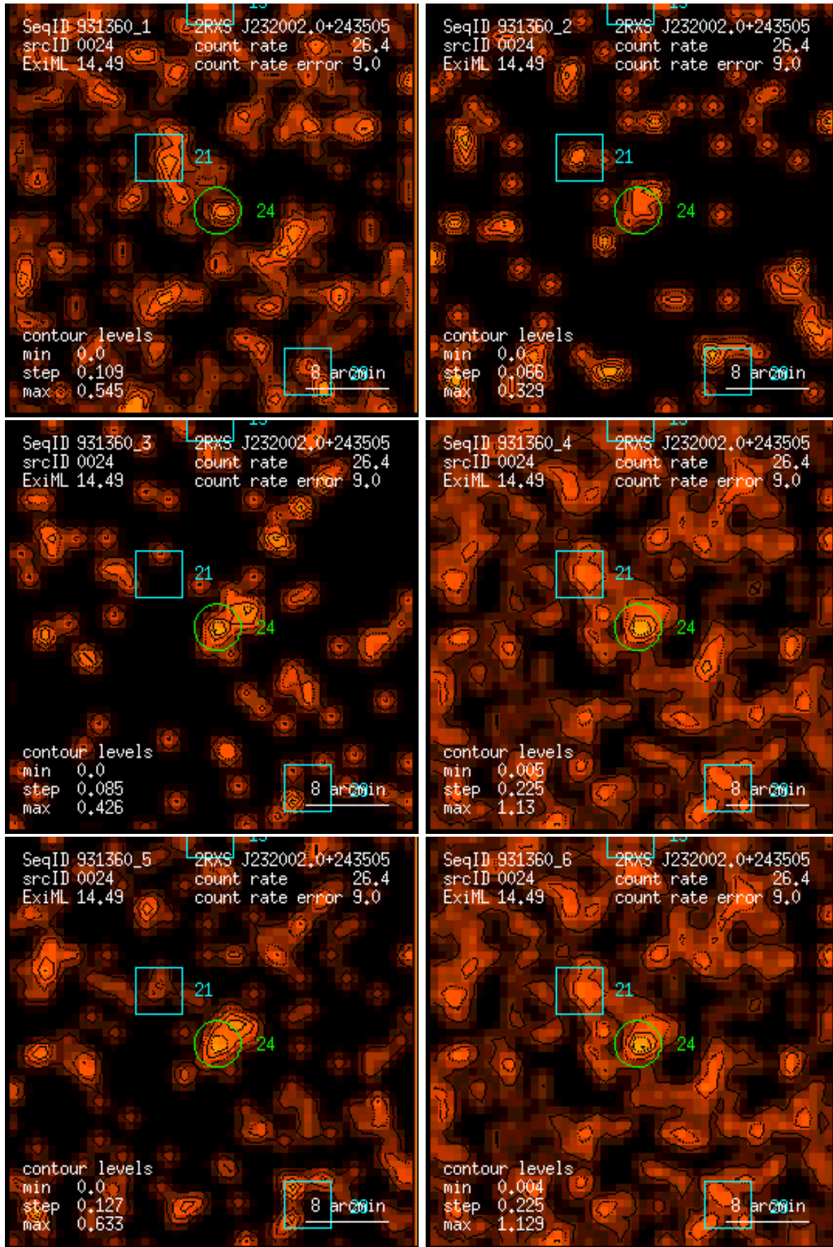
Figure 24: RASS 931360: detection 0024: band rate images, Gaussian filter: (1) PSPC channels 11 – 41, (2) 52 – 90, (3) 91 – 201, (4) 11 – 235, (5) 52 – 201, (6) 11 – 201. Broad band rates in counts/ks. Band rate contour levels in counts/ks/arcmin 2 .
