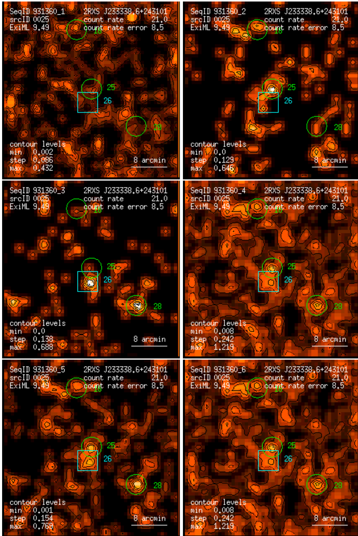
Figure 25: RASS 931360: detection 0025: band rate images, Gaussian filter: (1) PSPC channels 11 – 41, (2) 52 – 90, (3) 91 – 201, (4) 11 – 235, (5) 52 – 201, (6) 11 – 201. Broad band rates in counts/ks. Band rate contour levels in counts/ks/arcmin 2 .
