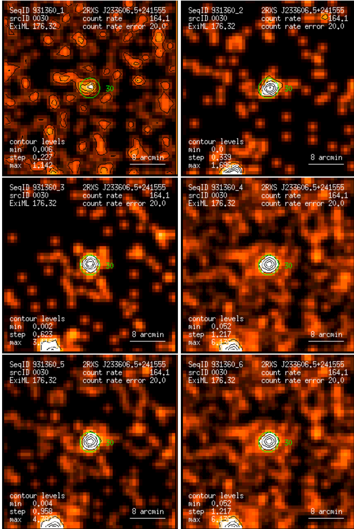
Figure 30: RASS 931360: detection 0030: band rate images, Gaussian filter: (1) PSPC channels 11 – 41, (2) 52 – 90, (3) 91 – 201, (4) 11 – 235, (5) 52 – 201, (6) 11 – 201. Broad band rates in counts/ks. Band rate contour levels in counts/ks/arcmin 2 .
