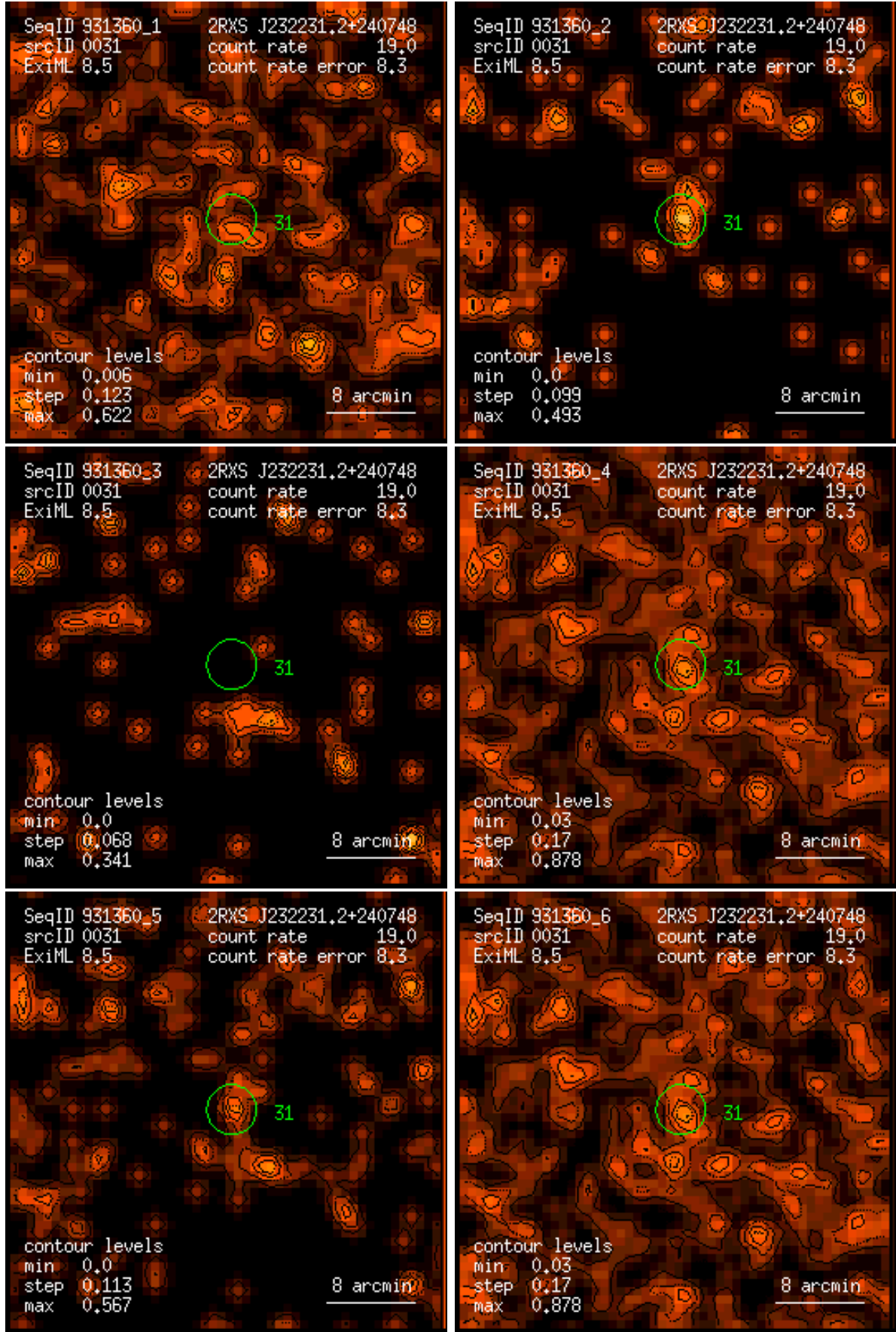
Figure 31: RASS 931360: detection 0031: band rate images, Gaussian filter: (1) PSPC channels 11 – 41, (2) 52 – 90, (3) 91 – 201, (4) 11 – 235, (5) 52 – 201, (6) 11 – 201. Broad band rates in counts/ks. Band rate contour levels in counts/ks/arcmin 2 .
