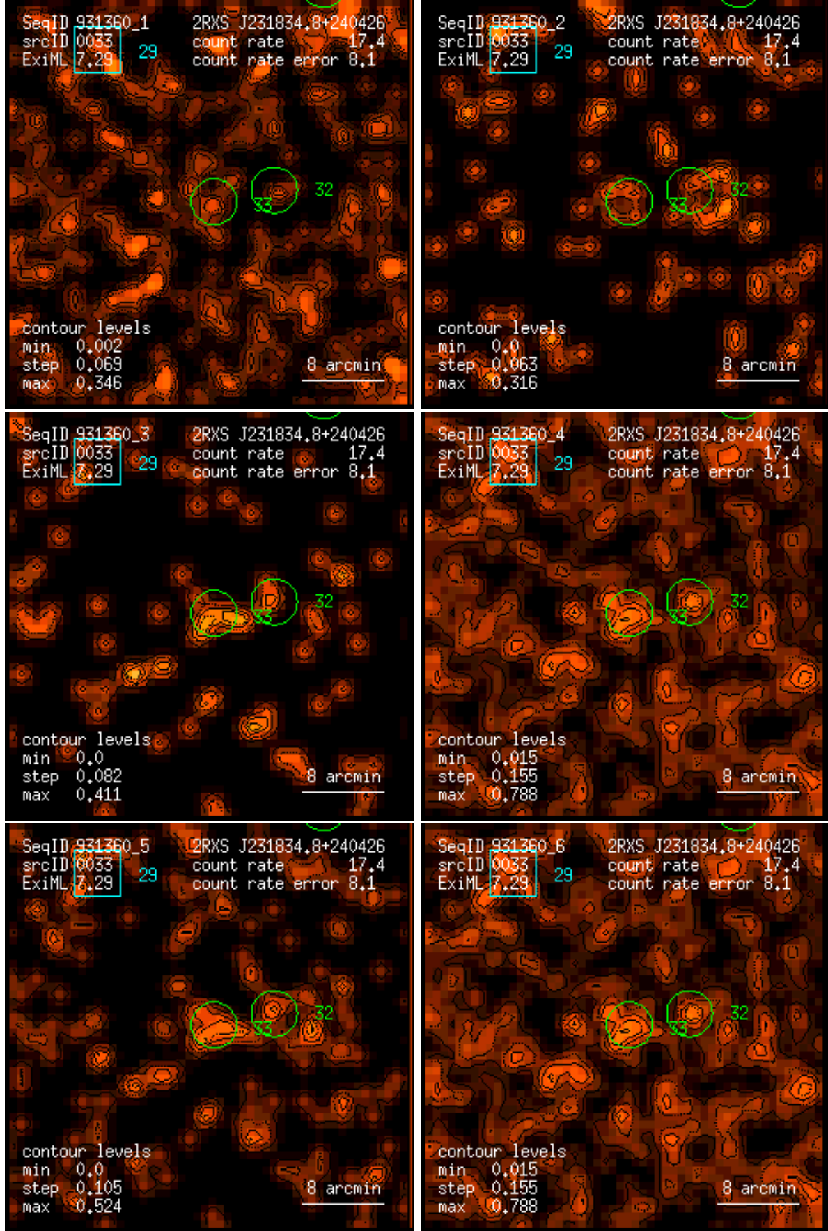
Figure 33: RASS 931360: detection 0033: band rate images, Gaussian filter: (1) PSPC channels 11 – 41, (2) 52 – 90, (3) 91 – 201, (4) 11 – 235, (5) 52 – 201, (6) 11 – 201. Broad band rates in counts/ks. Band rate contour levels in counts/ks/arcmin 2 .
