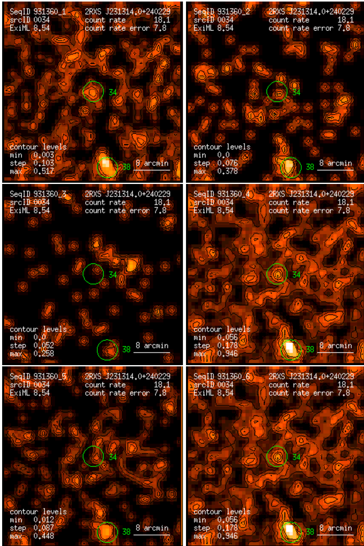
Figure 34: RASS 931360: detection 0034: band rate images, Gaussian filter: (1) PSPC channels 11 – 41, (2) 52 – 90, (3) 91 – 201, (4) 11 – 235, (5) 52 – 201, (6) 11 – 201. Broad band rates in counts/ks. Band rate contour levels in counts/ks/arcmin 2 .
