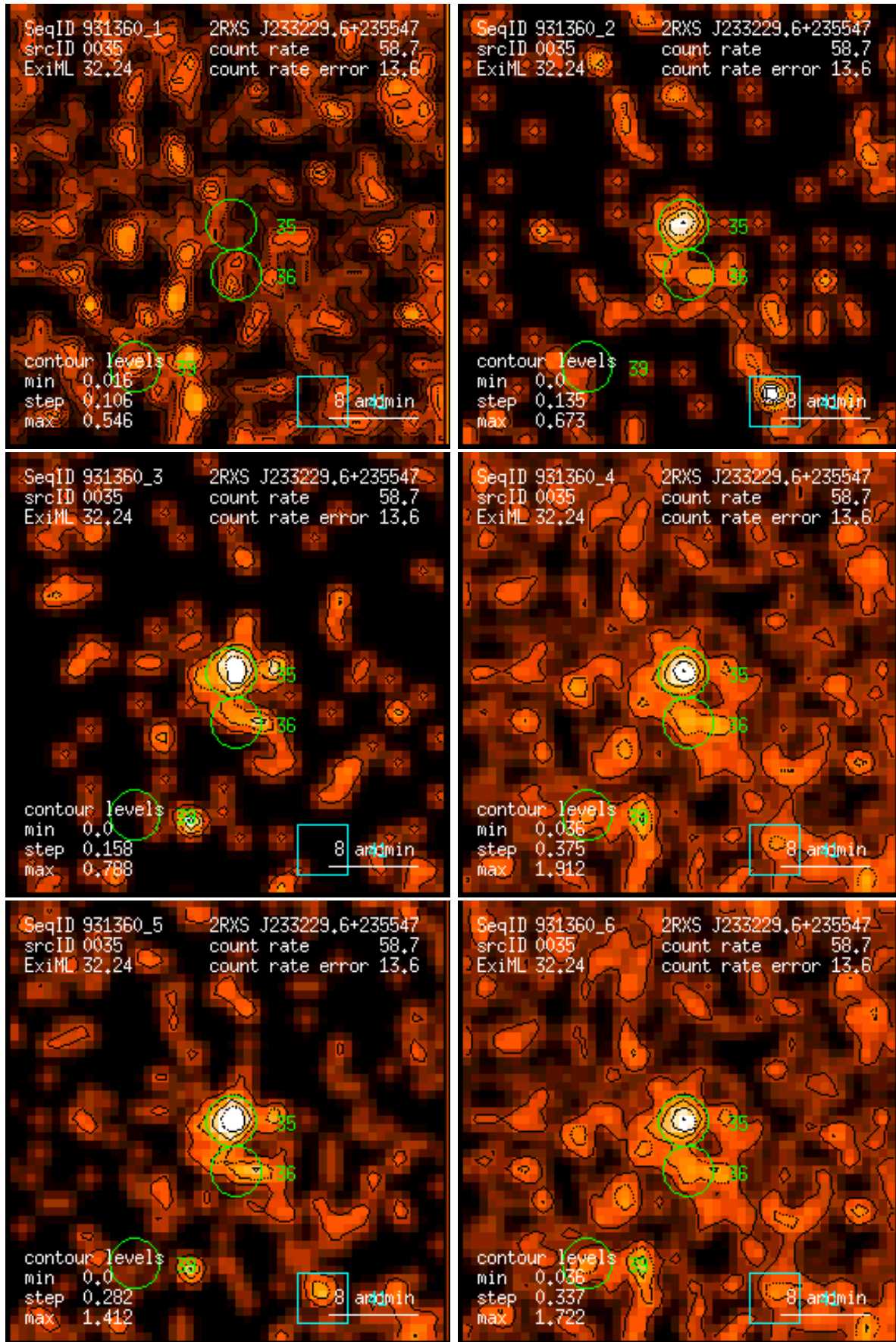
Figure 35: RASS 931360: detection 0035: band rate images, Gaussian filter: (1) PSPC channels 11 – 41, (2) 52 – 90, (3) 91 – 201, (4) 11 – 235, (5) 52 – 201, (6) 11 – 201. Broad band rates in counts/ks. Band rate contour levels in counts/ks/arcmin 2 .
