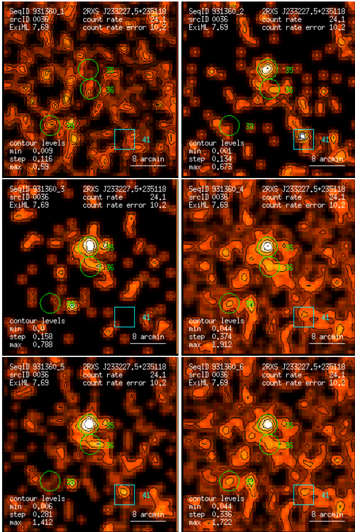
Figure 36: RASS 931360: detection 0036: band rate images, Gaussian filter: (1) PSPC channels 11 – 41, (2) 52 – 90, (3) 91 – 201, (4) 11 – 235, (5) 52 – 201, (6) 11 – 201. Broad band rates in counts/ks. Band rate contour levels in counts/ks/arcmin 2 .
