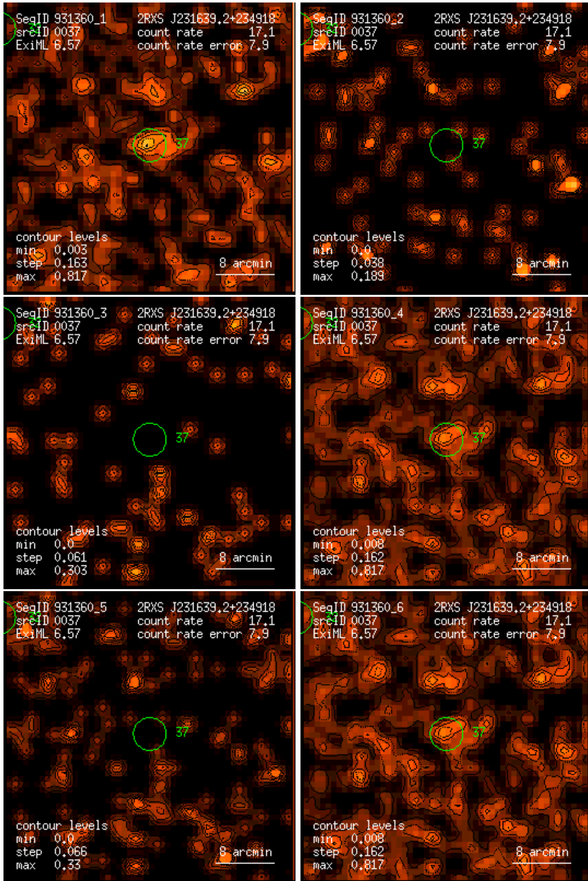
Figure 37: RASS 931360: detection 0037: band rate images, Gaussian filter: (1) PSPC channels 11 – 41, (2) 52 – 90, (3) 91 – 201, (4) 11 – 235, (5) 52 – 201, (6) 11 – 201. Broad band rates in counts/ks. Band rate contour levels in counts/ks/arcmin 2 .
