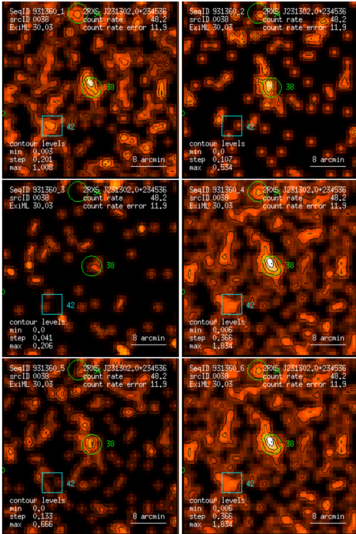
Figure 38: RASS 931360: detection 0038: band rate images, Gaussian filter: (1) PSPC channels 11 – 41, (2) 52 – 90, (3) 91 – 201, (4) 11 – 235, (5) 52 – 201, (6) 11 – 201. Broad band rates in counts/ks. Band rate contour levels in counts/ks/arcmin 2 .
