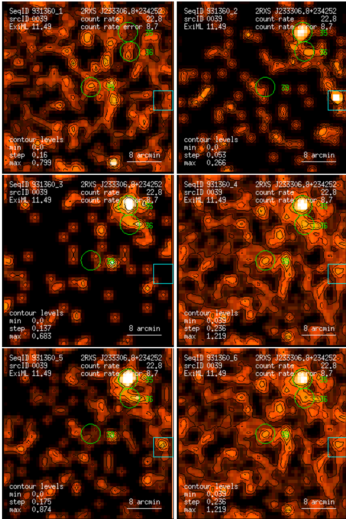
Figure 39: RASS 931360: detection 0039: band rate images, Gaussian filter: (1) PSPC channels 11 – 41, (2) 52 – 90, (3) 91 – 201, (4) 11 – 235, (5) 52 – 201, (6) 11 – 201. Broad band rates in counts/ks. Band rate contour levels in counts/ks/arcmin 2 .
