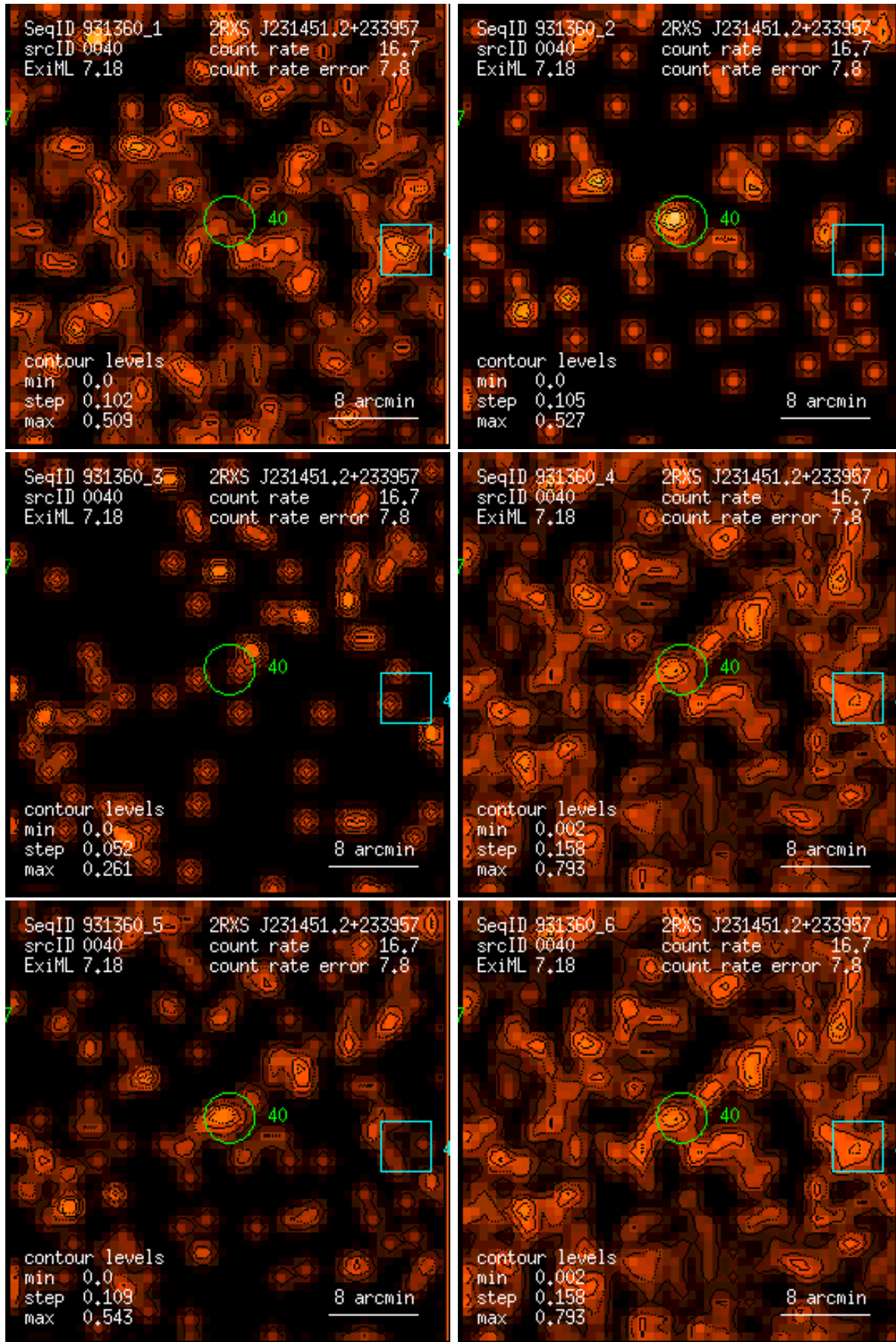
Figure 40: RASS 931360: detection 0040: band rate images, Gaussian filter: (1) PSPC channels 11 – 41, (2) 52 – 90, (3) 91 – 201, (4) 11 – 235, (5) 52 – 201, (6) 11 – 201. Broad band rates in counts/ks. Band rate contour levels in counts/ks/arcmin 2 .
