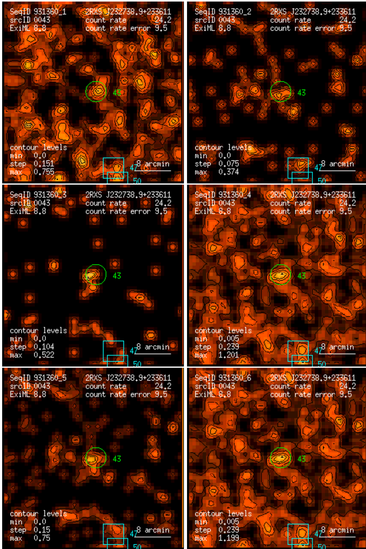
Figure 43: RASS 931360: detection 0043: band rate images, Gaussian filter: (1) PSPC channels 11 – 41, (2) 52 – 90, (3) 91 – 201, (4) 11 – 235, (5) 52 – 201, (6) 11 – 201. Broad band rates in counts/ks. Band rate contour levels in counts/ks/arcmin 2 .
