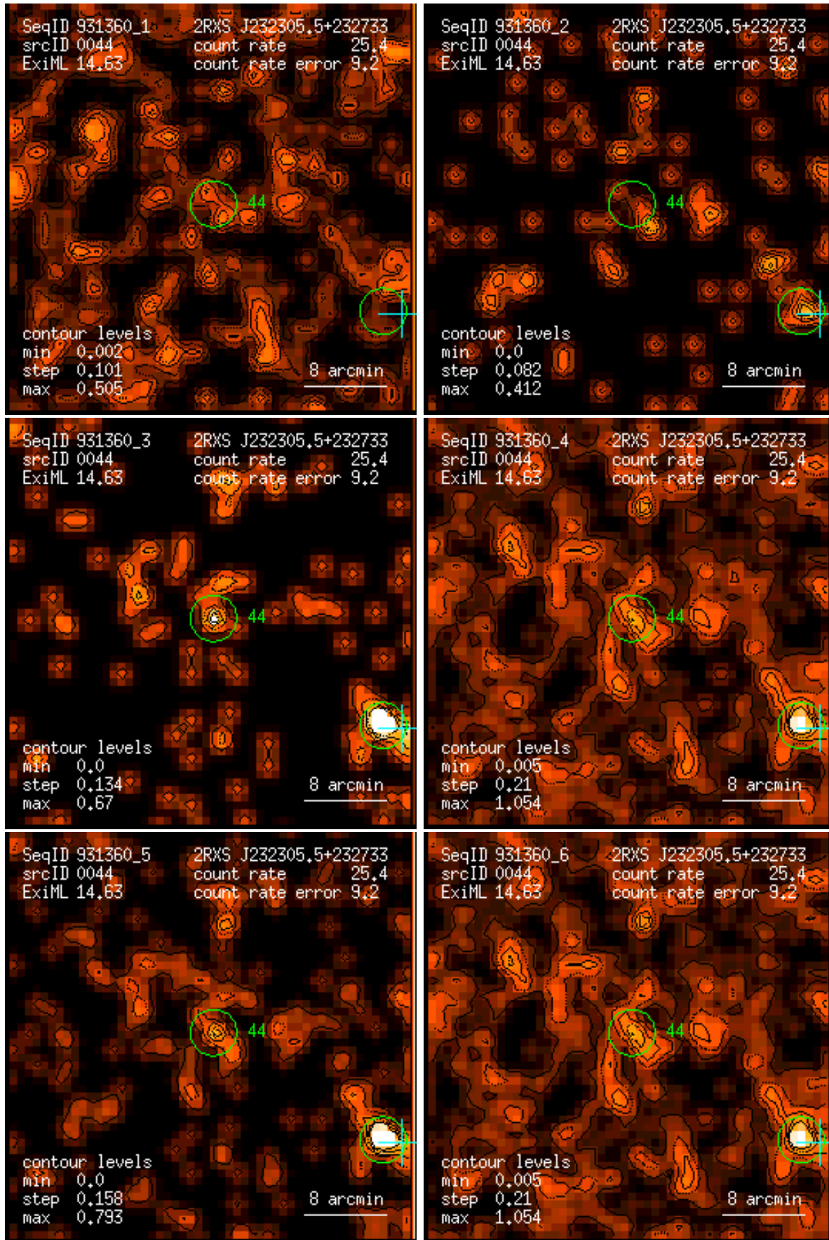
Figure 44: RASS 931360: detection 0044: band rate images, Gaussian filter: (1) PSPC channels 11 – 41, (2) 52 – 90, (3) 91 – 201, (4) 11 – 235, (5) 52 – 201, (6) 11 – 201. Broad band rates in counts/ks. Band rate contour levels in counts/ks/arcmin 2 .
