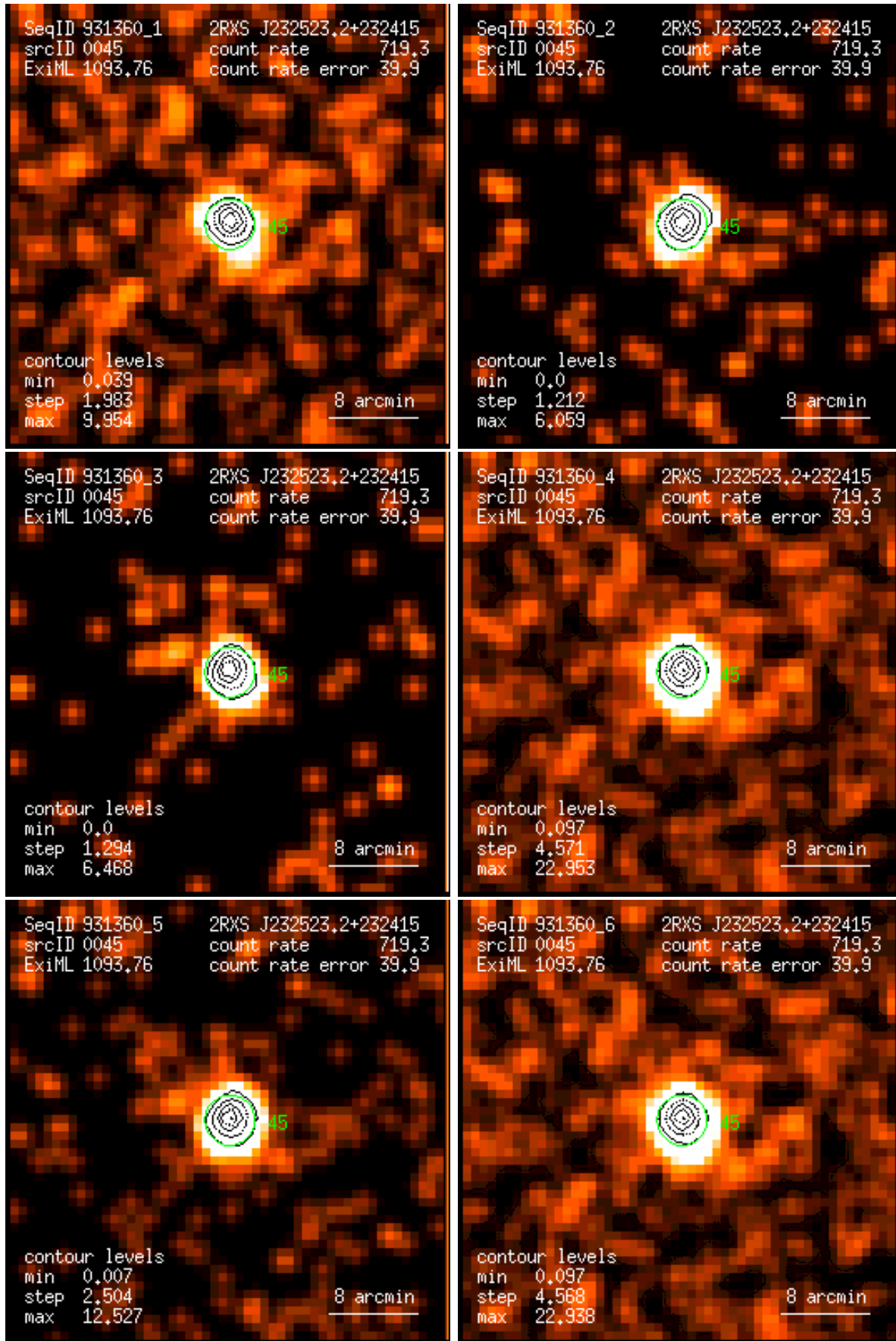
Figure 45: RASS 931360: detection 0045: band rate images, Gaussian filter: (1) PSPC channels 11 – 41, (2) 52 – 90, (3) 91 – 201, (4) 11 – 235, (5) 52 – 201, (6) 11 – 201. Broad band rates in counts/ks. Band rate contour levels in counts/ks/arcmin 2 .
