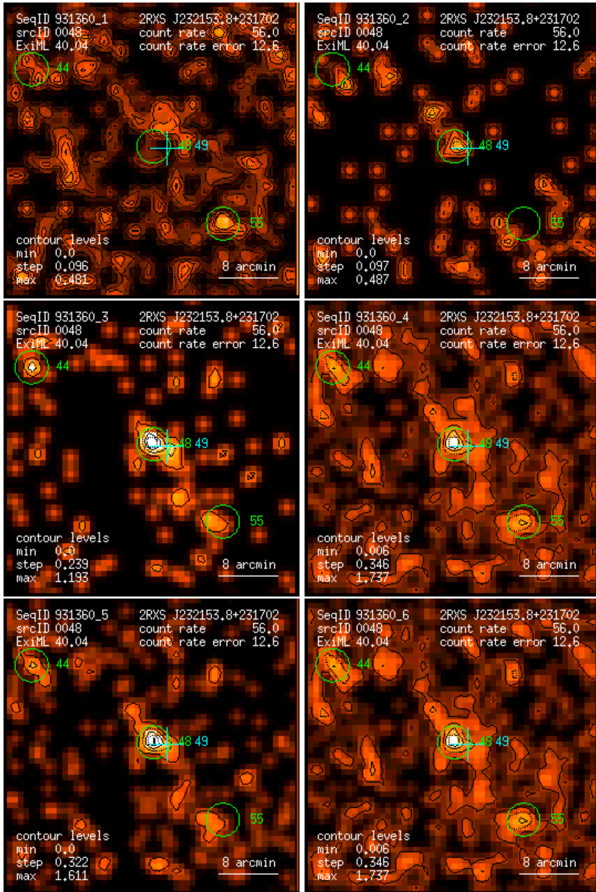
Figure 48: RASS 931360: detection 0048: band rate images, Gaussian filter: (1) PSPC channels 11 – 41, (2) 52 – 90, (3) 91 – 201, (4) 11 – 235, (5) 52 – 201, (6) 11 – 201. Broad band rates in counts/ks. Band rate contour levels in counts/ks/arcmin 2 .
