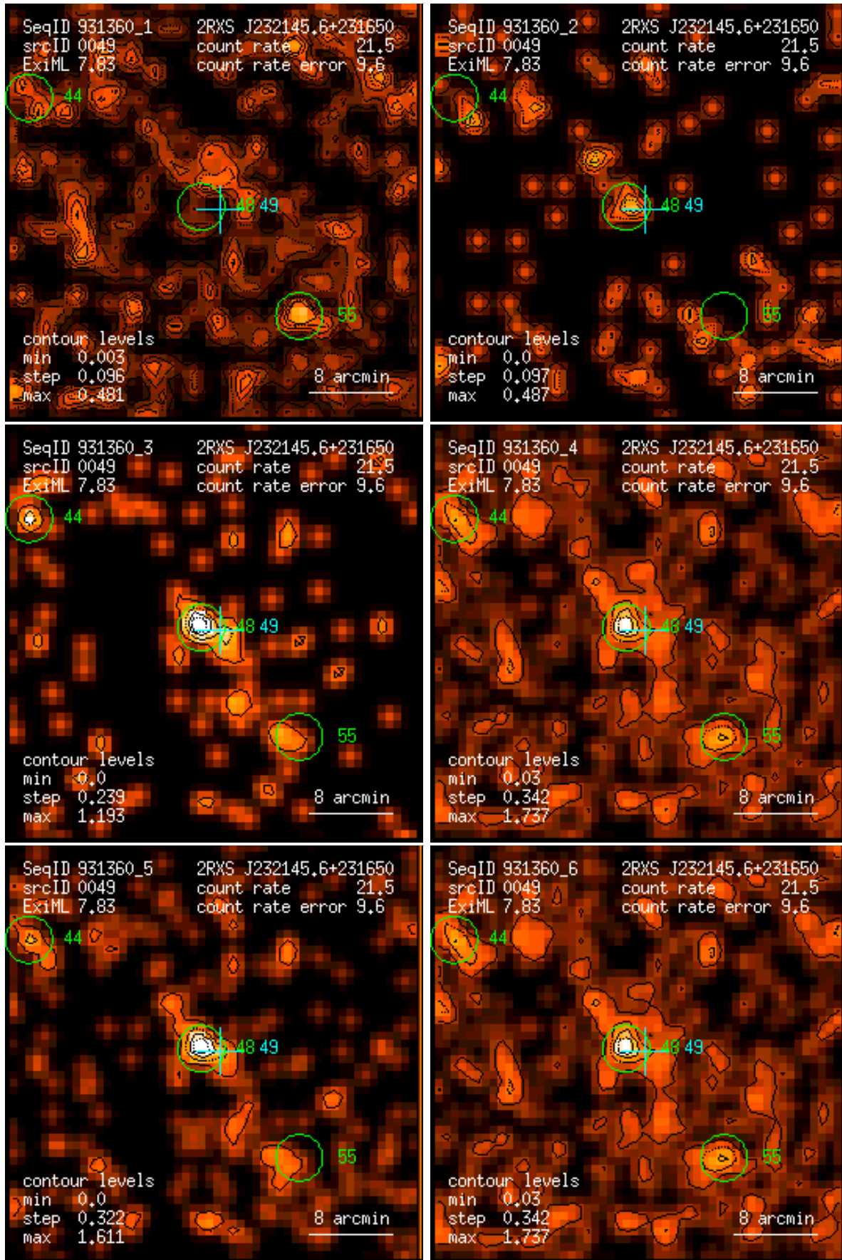
Figure 49: RASS 931360: detection 0049: band rate images, Gaussian filter: (1) PSPC channels 11 – 41, (2) 52 – 90, (3) 91 – 201, (4) 11 – 235, (5) 52 – 201, (6) 11 – 201. Broad band rates in counts/ks. Band rate contour levels in counts/ks/arcmin 2 .
