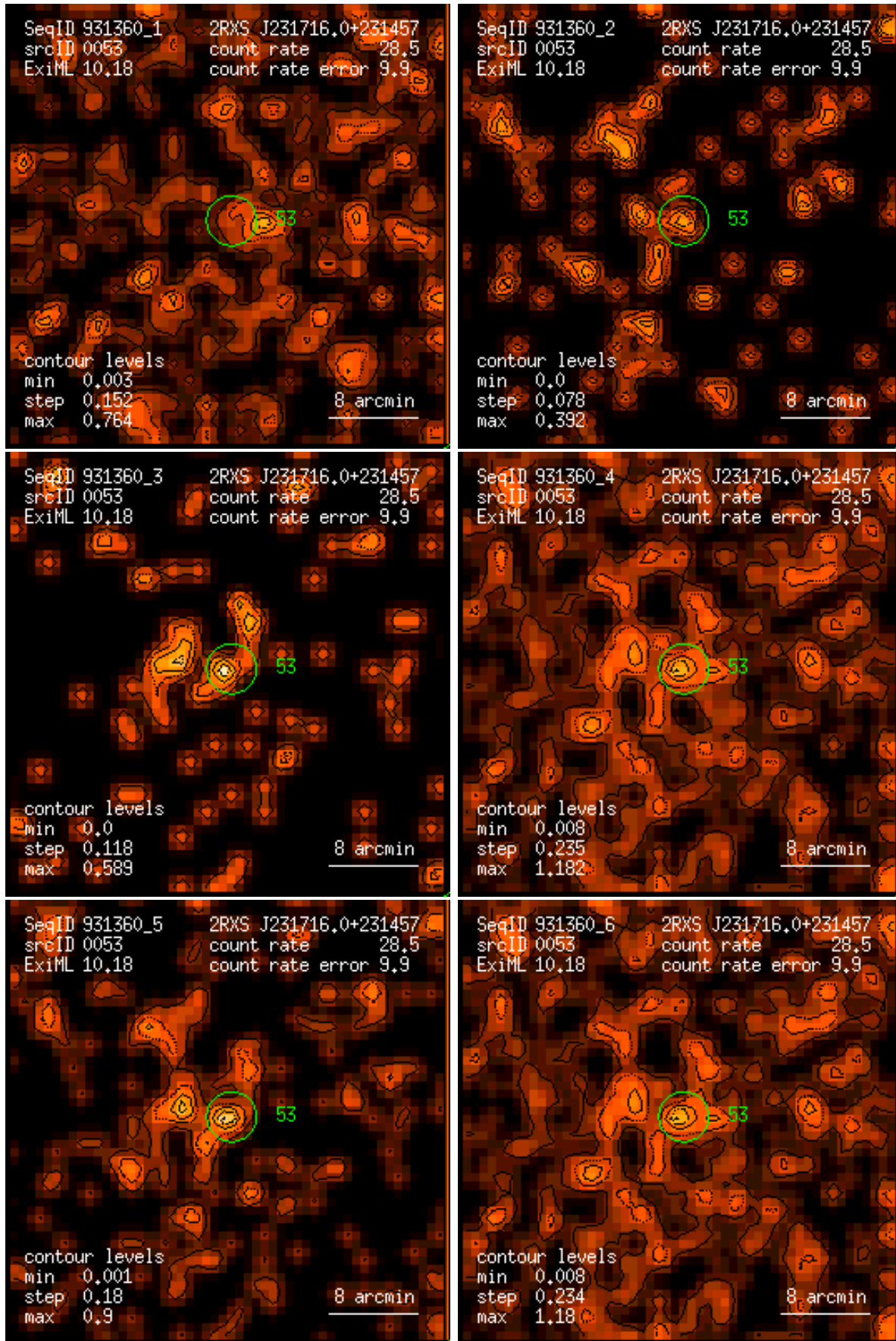
Figure 53: RASS 931360: detection 0053: band rate images, Gaussian filter: (1) PSPC channels 11 – 41, (2) 52 – 90, (3) 91 – 201, (4) 11 – 235, (5) 52 – 201, (6) 11 – 201. Broad band rates in counts/ks. Band rate contour levels in counts/ks/arcmin 2 .
