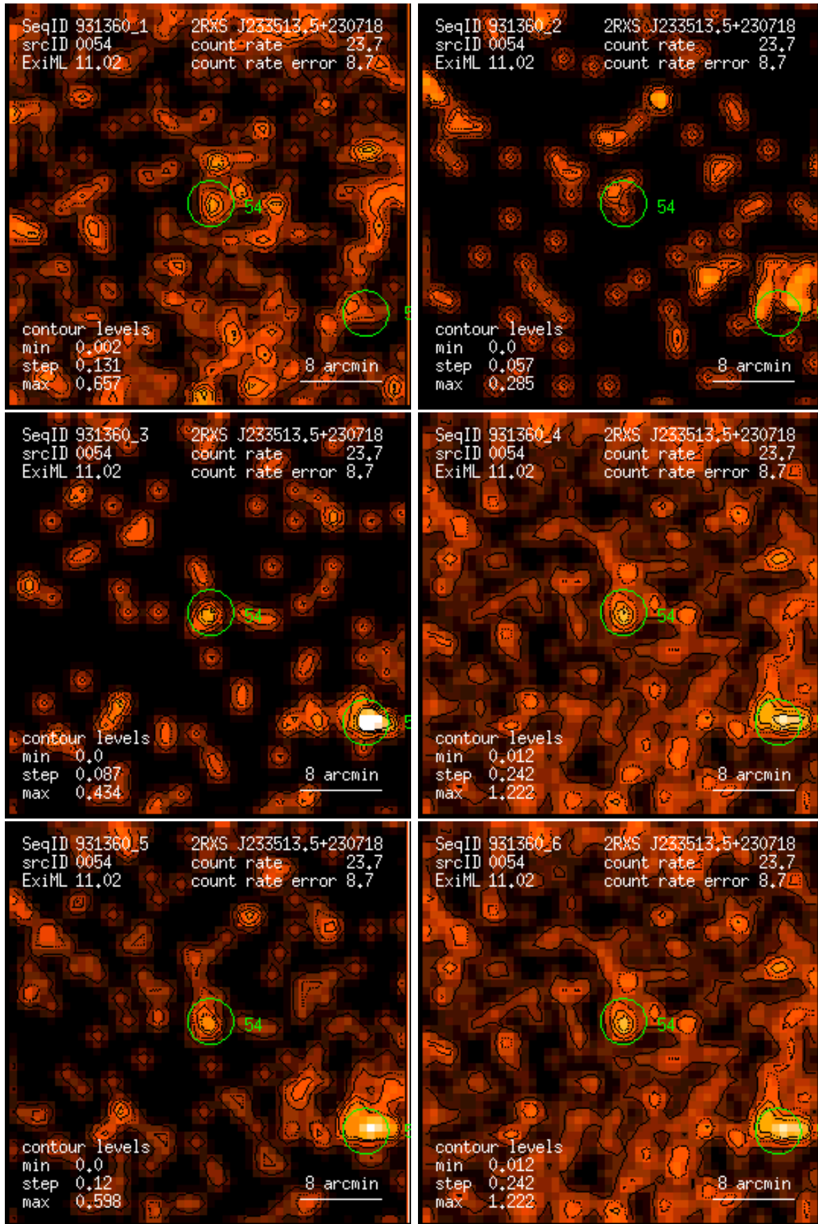
Figure 54: RASS 931360: detection 0054: band rate images, Gaussian filter: (1) PSPC channels 11 – 41, (2) 52 – 90, (3) 91 – 201, (4) 11 – 235, (5) 52 – 201, (6) 11 – 201. Broad band rates in counts/ks. Band rate contour levels in counts/ks/arcmin 2 .
