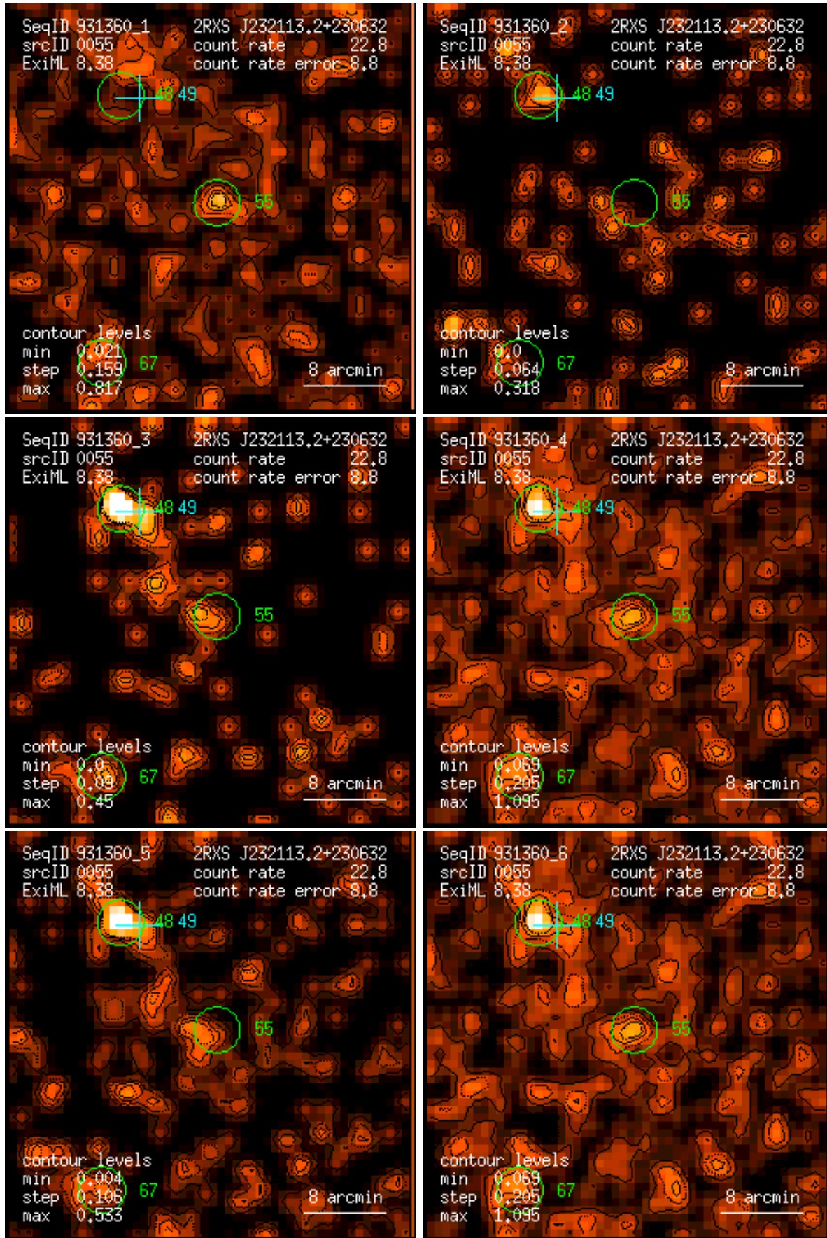
Figure 55: RASS 931360: detection 0055: band rate images, Gaussian filter: (1) PSPC channels 11 – 41, (2) 52 – 90, (3) 91 – 201, (4) 11 – 235, (5) 52 – 201, (6) 11 – 201. Broad band rates in counts/ks. Band rate contour levels in counts/ks/arcmin 2 .
