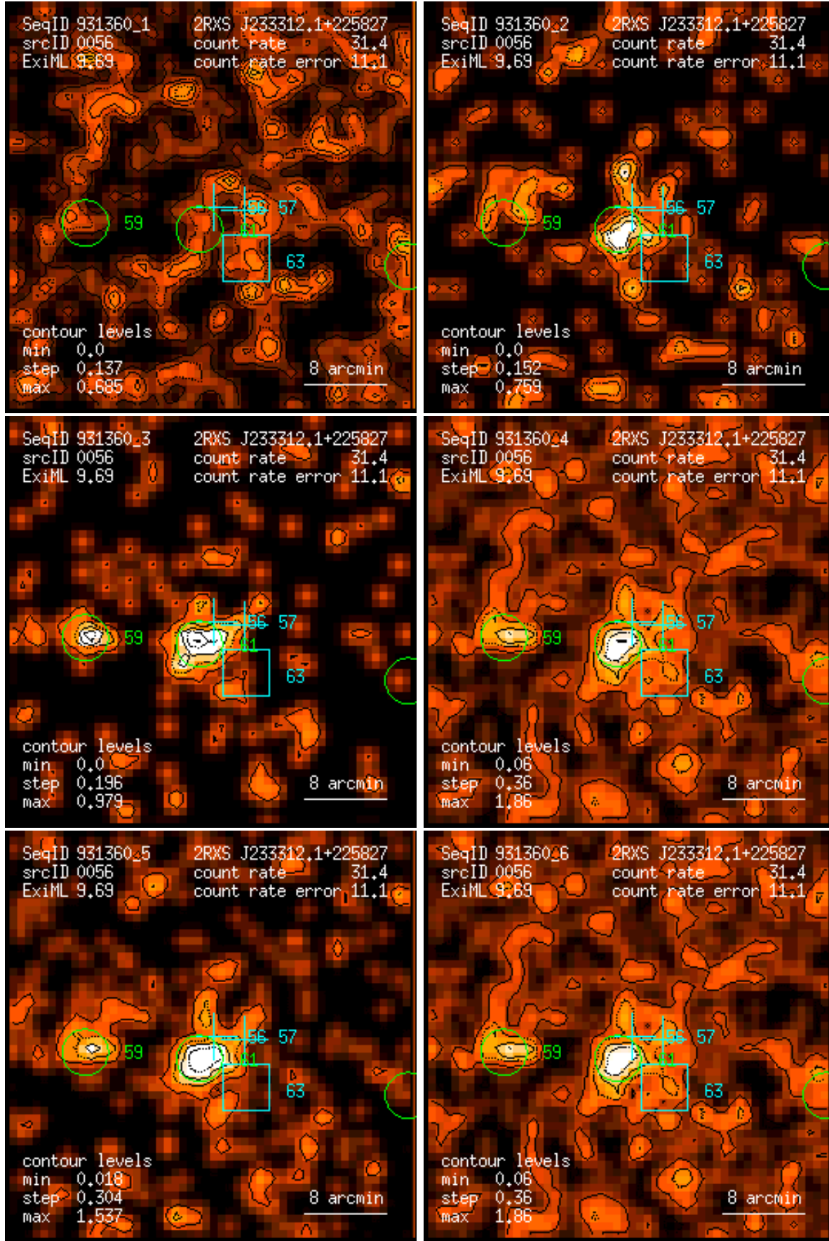
Figure 56: RASS 931360: detection 0056: band rate images, Gaussian filter: (1) PSPC channels 11 – 41, (2) 52 – 90, (3) 91 – 201, (4) 11 – 235, (5) 52 – 201, (6) 11 – 201. Broad band rates in counts/ks. Band rate contour levels in counts/ks/arcmin 2 .
