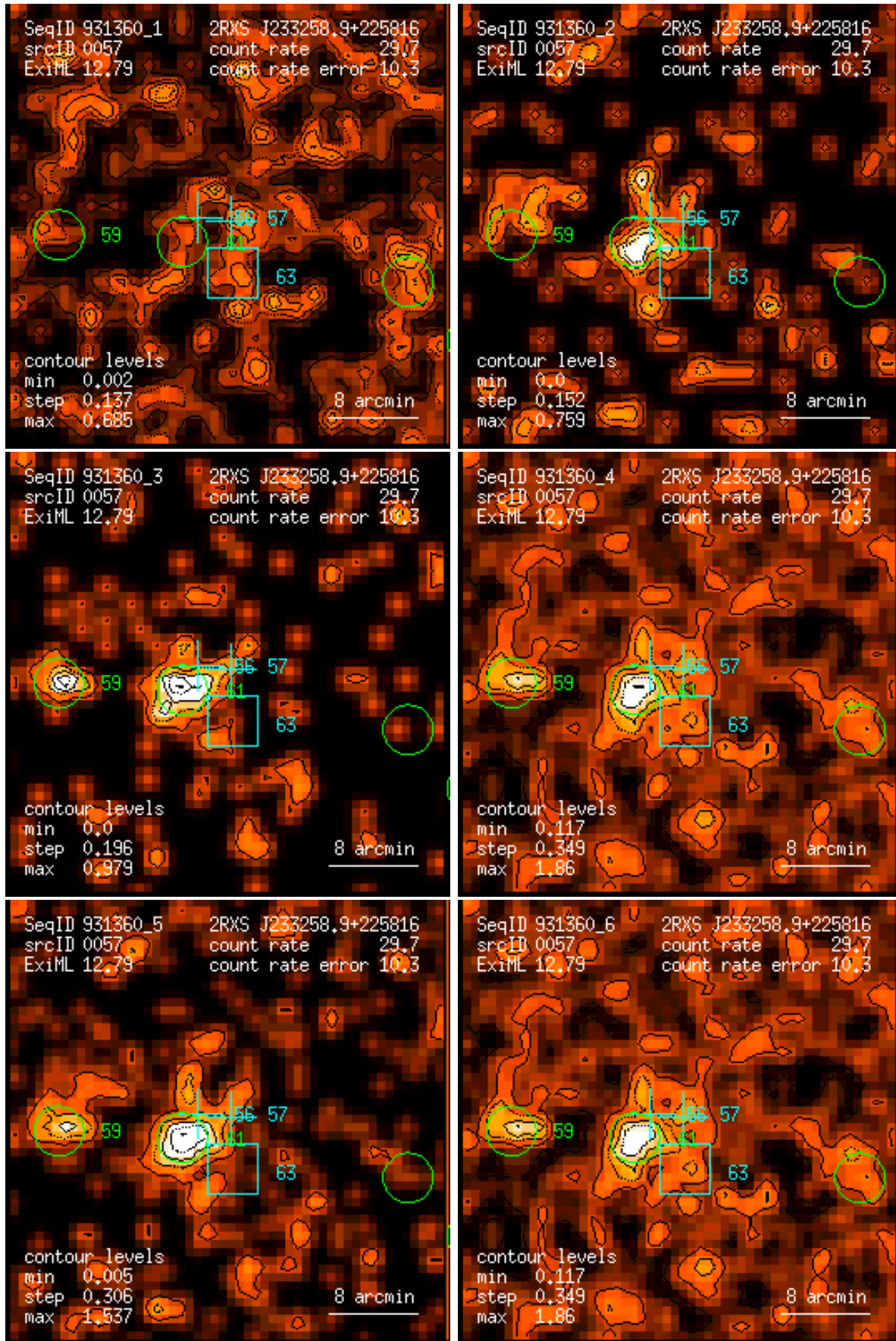
Figure 57: RASS 931360: detection 0057: band rate images, Gaussian filter: (1) PSPC channels 11 – 41, (2) 52 – 90, (3) 91 – 201, (4) 11 – 235, (5) 52 – 201, (6) 11 – 201. Broad band rates in counts/ks. Band rate contour levels in counts/ks/arcmin 2 .
