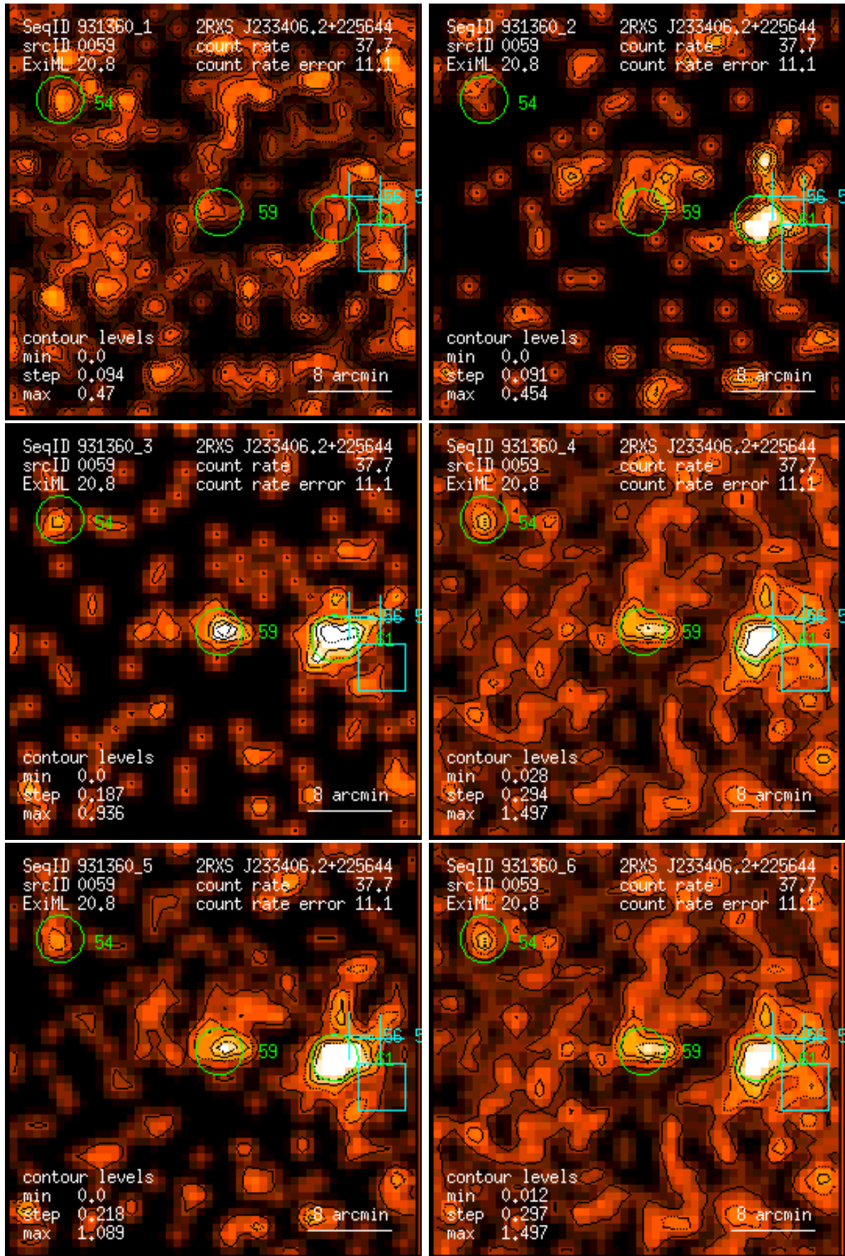
Figure 59: RASS 931360: detection 0059: band rate images, Gaussian filter: (1) PSPC channels 11 – 41, (2) 52 – 90, (3) 91 – 201, (4) 11 – 235, (5) 52 – 201, (6) 11 – 201. Broad band rates in counts/ks. Band rate contour levels in counts/ks/arcmin 2 .
