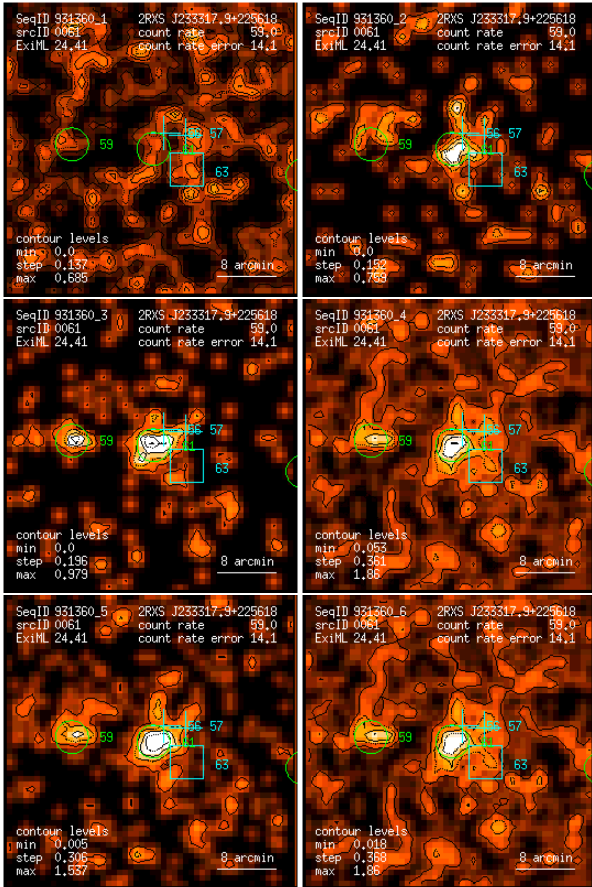
Figure 61: RASS 931360: detection 0061: band rate images, Gaussian filter: (1) PSPC channels 11 – 41, (2) 52 – 90, (3) 91 – 201, (4) 11 – 235, (5) 52 – 201, (6) 11 – 201. Broad band rates in counts/ks. Band rate contour levels in counts/ks/arcmin 2 .
